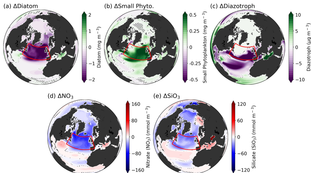
Figure 2. (a–c) Differences in each PFT between CO 2 down and climatology periods (d–e), Differences in macronutrients (NO 3 , SiO 3 ) between CO 2 down and climatology periods. Hatches indicate the non-significant region between total ensembles based on the bootstrap method.
