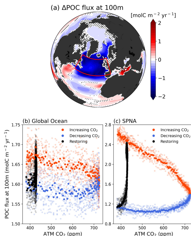
Figure 4. (a) Differences of Particulate Organic Carbon (POC) flux at 100 m depth between CO 2 down and climatology periods. Changes in POC flux at 100 m depth of (b), global ocean and (c), SPNA region in response to CO 2 forcing. Orange color scatters indicate the CO 2 increasing period, blue scatters indicate the CO 2 decreasing period and black scatters indicate the Restoring period.
