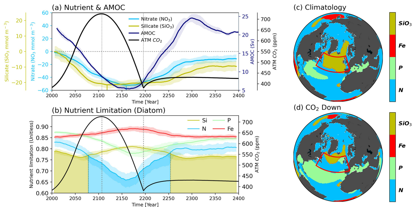
Figure 3. (a) Time series of strength of Atlantic Meridional Overturning Circulation (AMOC; navy), Nitrate (NO 3 ; sky-blue), Silicate (SiO 3 ; dark-khaki) and atmospheric CO 2 concentration (black) (b), Nutrient limitation of diatom for four nutrients (SiO 3 ; dark-khaki, Nitrogen (N); sky-blue, Phosphorus (P); light-green, Iron (Fe); red). All plots are drawn in 11-year moving averages and the shading indicates the range of minimum-maximum values between total ensembles. In addition, the shaded areas under the plots indicate the primary limiting nutrients for diatom growth. Nutrient limitation distribution of diatom during both (c) Climatology and (d) CO 2 down period.
