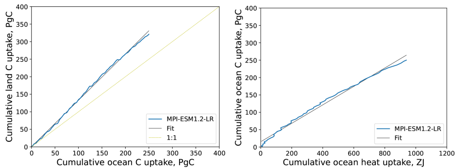
Figure 3. Results of the flat10 experiment with MPI-ESM1.2-LR (blue lines). Left: dynamics of cumulative land vs. ocean carbon uptakes. Right: changes in cumulative ocean carbon and heat uptakes. Black lines are for linear fits.
