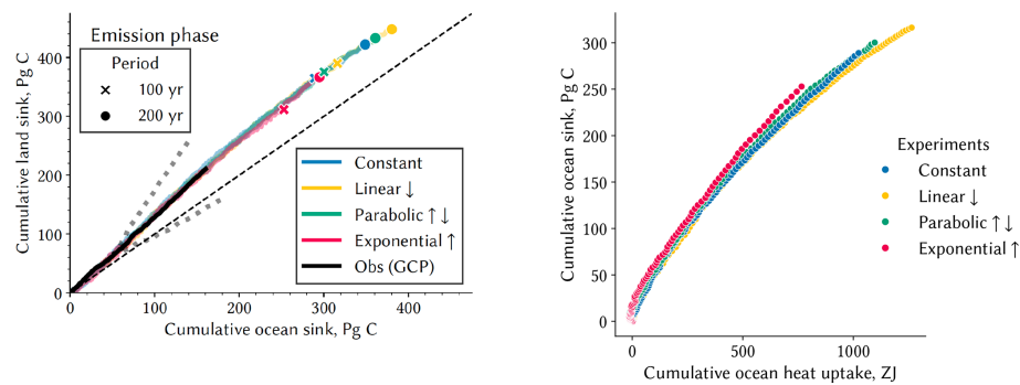
Figure A2. In MPI-ESM simulations with total CO 2 emissions of 1200 Pg C for 100 or 200 years, the sink shares of land versus ocean (left) emerge to keep the same relationship irrespective of pathway profiles. The same is valid for ocean carbon vs. heat uptake (right). For details, see paper by Winkler et al. (2024).
