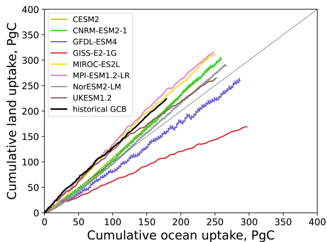
Figure 1. Cumulative land vs. ocean carbon uptakes in the flat10 experiments for the first 100 years. Historical land vs. ocean carbon sinks in the Global Carbon Budget (GCB) (Friedlingstein et al., 2023) for the period 1850–2022 are shown by continuous black line. The land sink in GCB is calculated from simulations in which \text{CO}_2 and climate evolved over the historical period, while the land cover stayed at its pre-industrial level (no land use change). The thin dash line is the 1 : 1 ratio.
