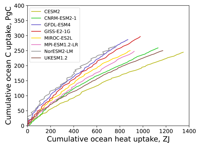
Figure 2. Changes in cumulative ocean carbon (PgC) and heat uptakes (Zeta Joules) in the flat10 experiments.
