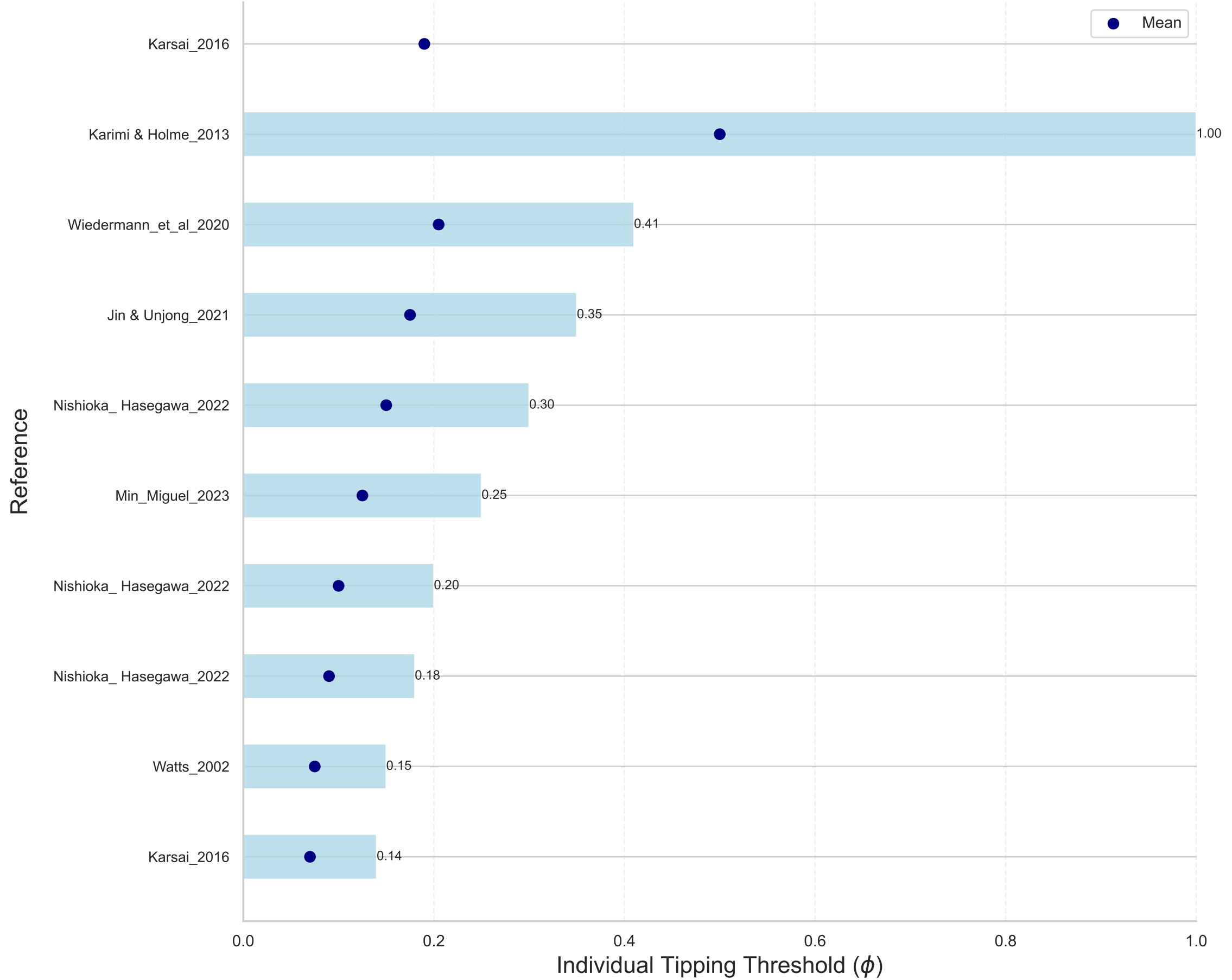
Threshold Fraction Ranges that Allow Tipping
