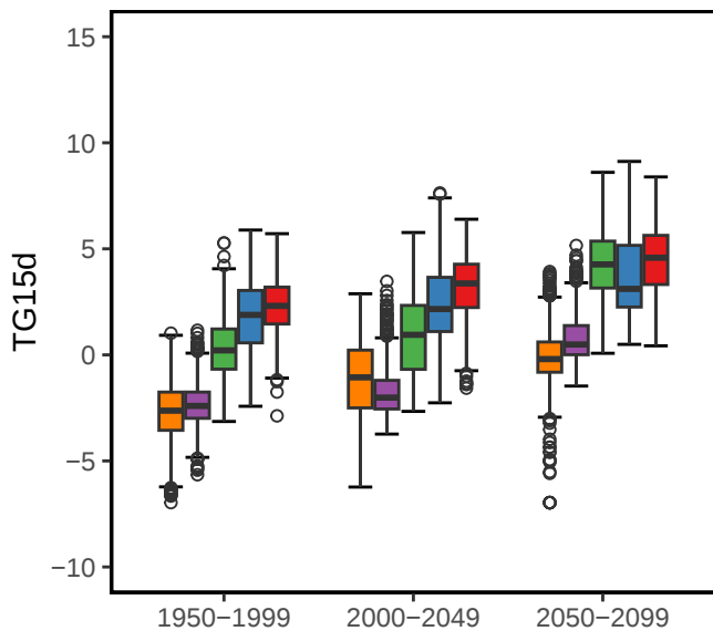
(c) SSP3-7.0
