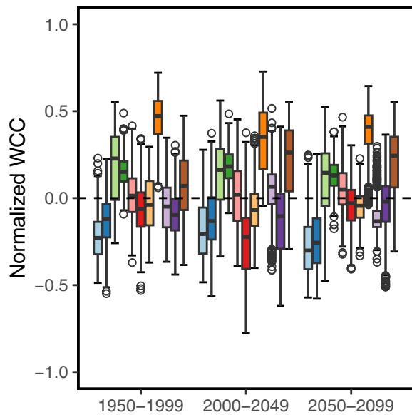
(c) SSP3-7.0
