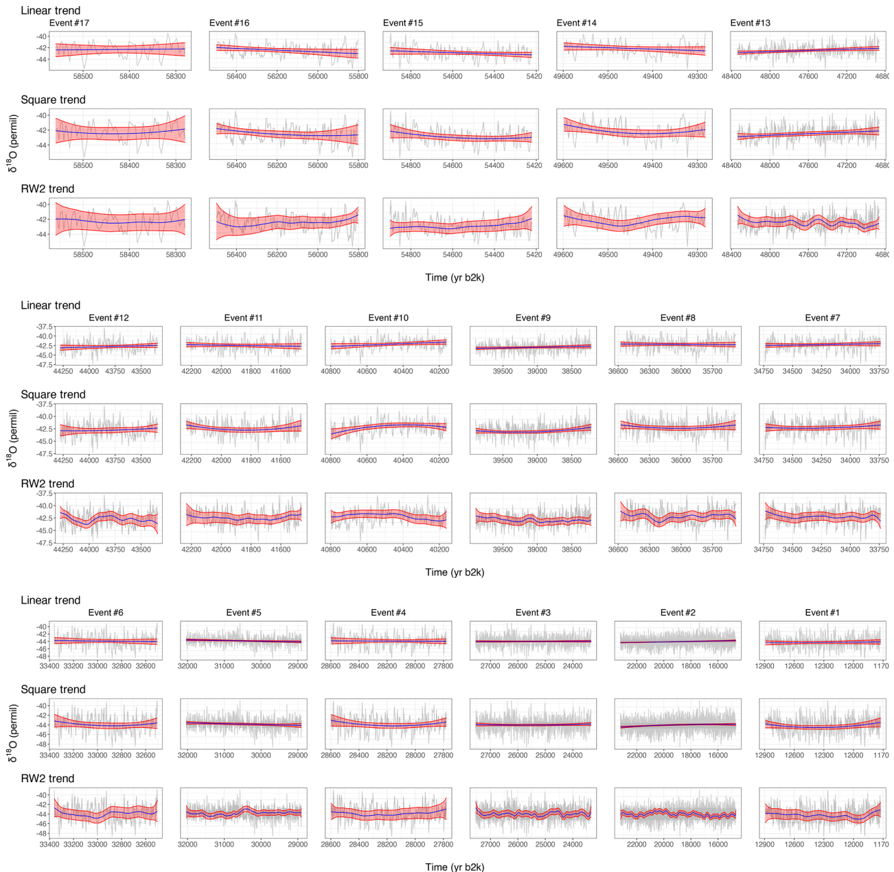
Figure C1. \delta^{18}\text{O} proxy data from the NGRIP record (gray), with Greenland stadial phases highlighted. The posterior marginal mean (blue) and 95 % credible intervals (red) of the fitted trends are included for each event.
