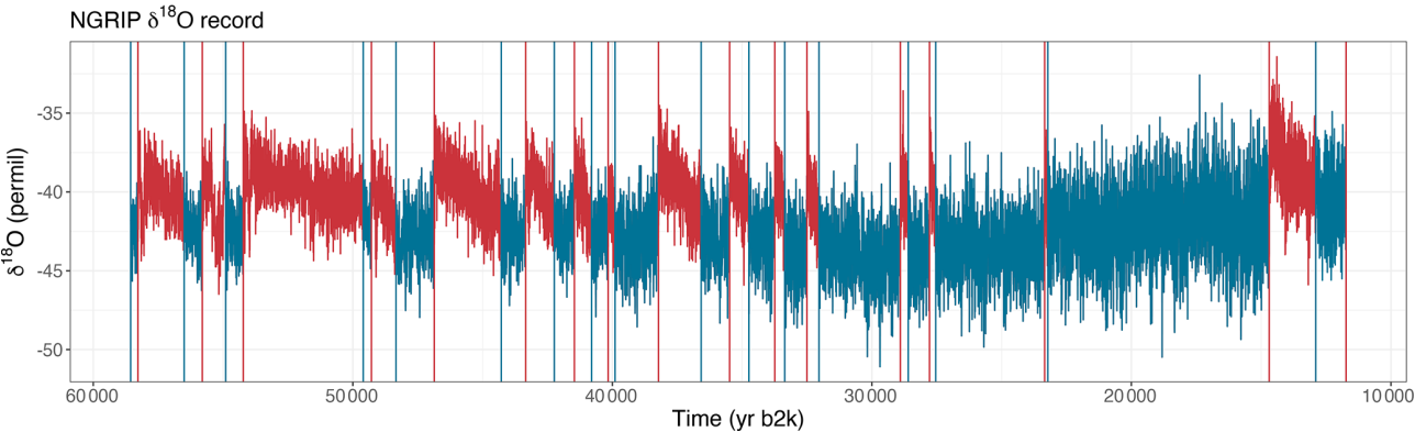
Figure 4. NGRIP \delta^{18}\text{O} proxy record. The time series used in our study are the parts of the curves drawn in turquoise, which are the cold stadial periods preceding the onsets of interstadial periods drawn in red. The red and turquoise vertical bars represent the start and end points of the interstadial periods, respectively.
