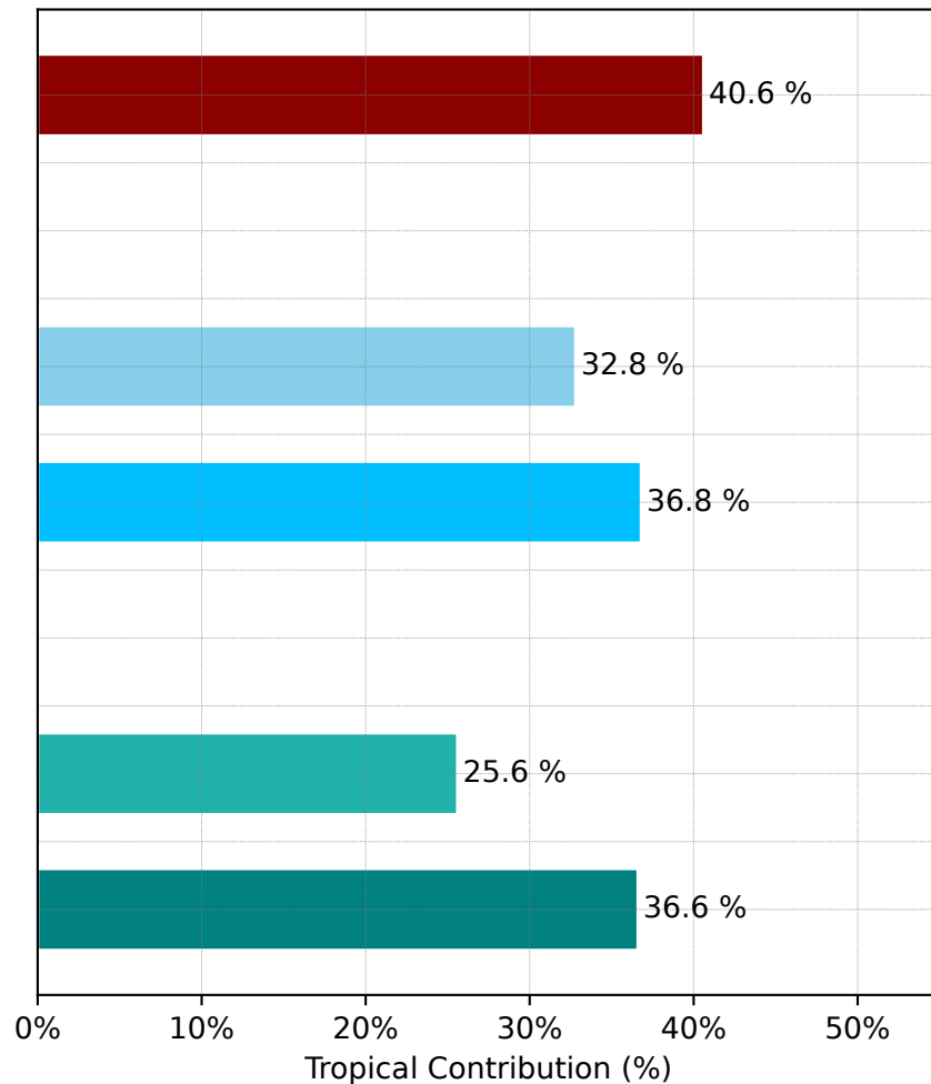
(b) FLEXPART-ERA5 trajectories
