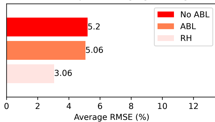
(b) \Delta t = 6 h, \Delta q_{min} = 0.2 g/kg, average
