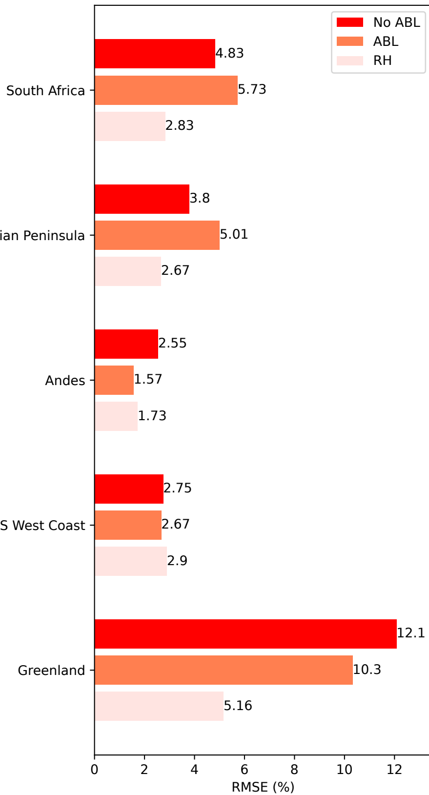
(b) \Delta t = 6 h, \Delta q_{min} = 0.2 g/kg, average
