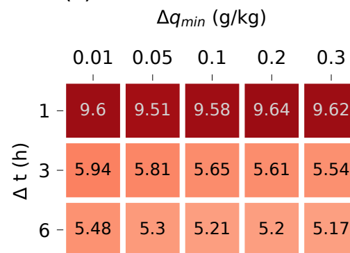
(c) No ABL
