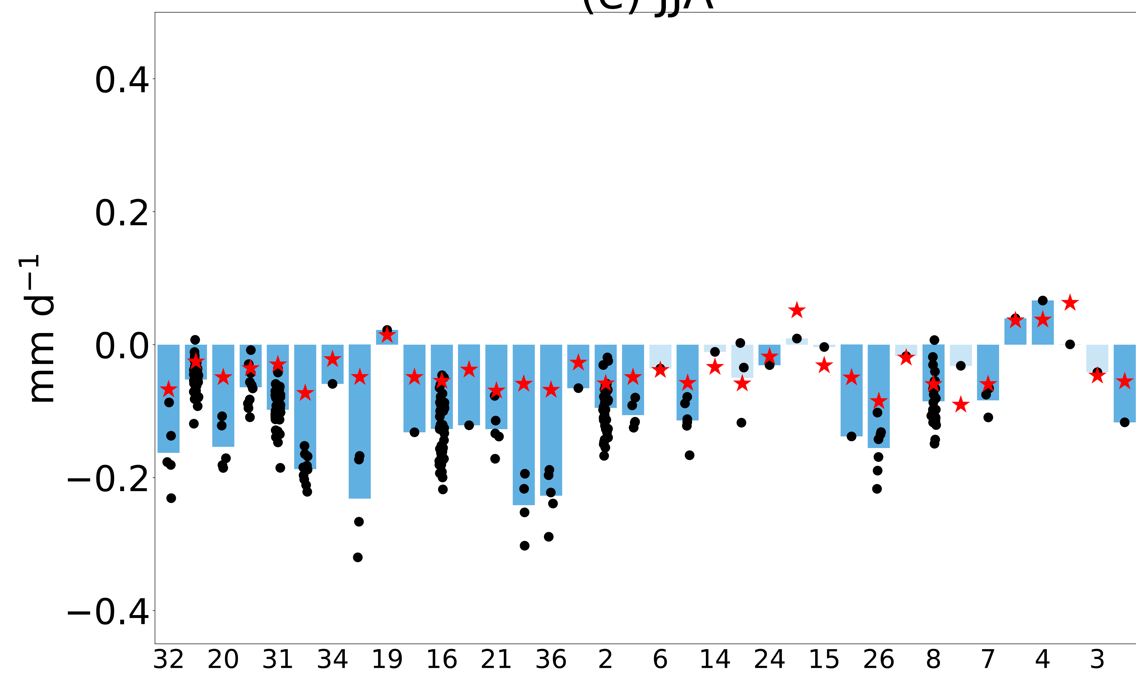
(e) JJA
