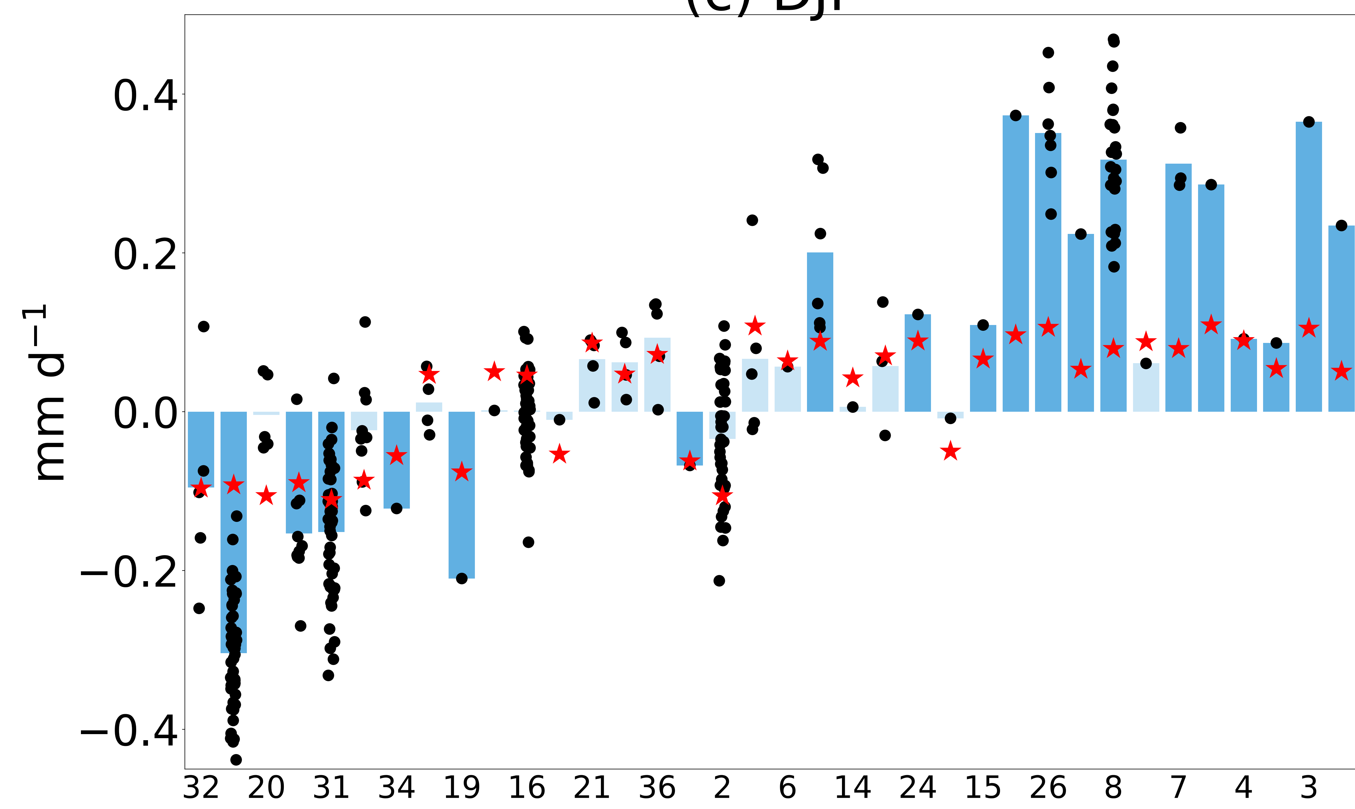
(c) DJF
