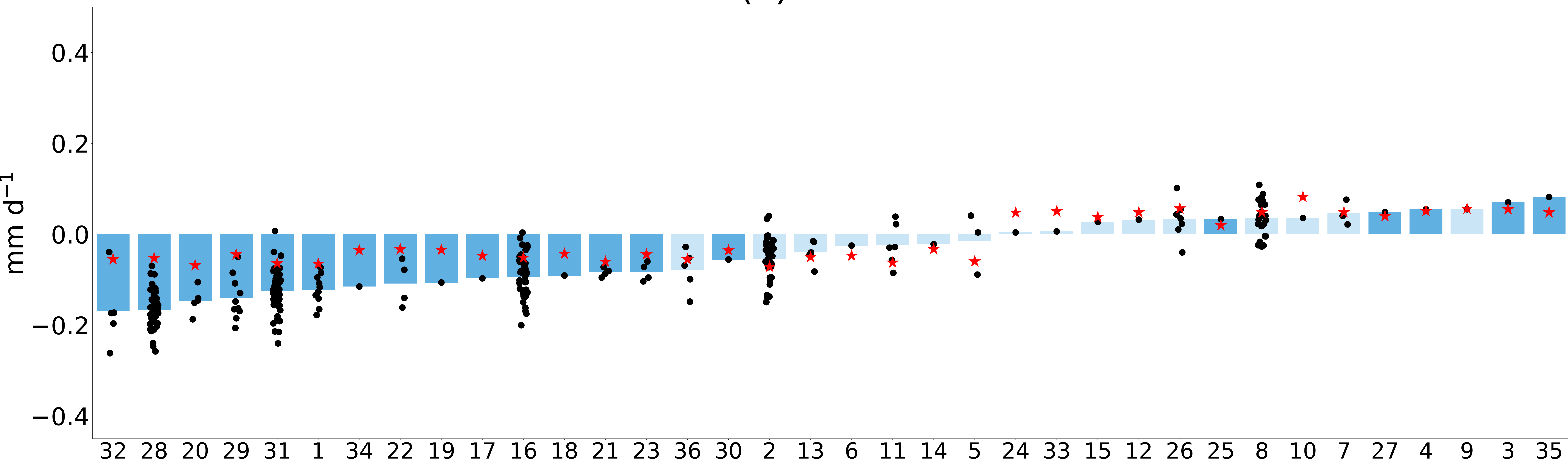
(a) Annual
