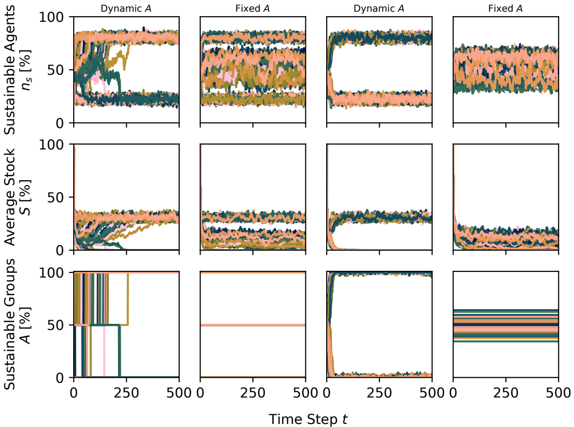
2 Groups with \sim 200 members ( N_g = 2 , N_m = 1 )
