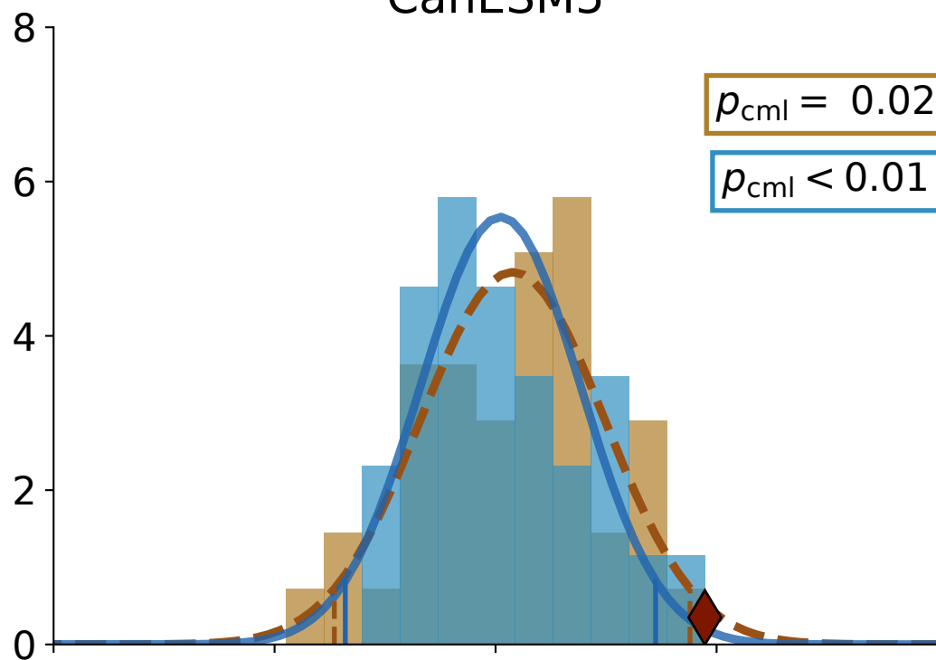
CanESM5
