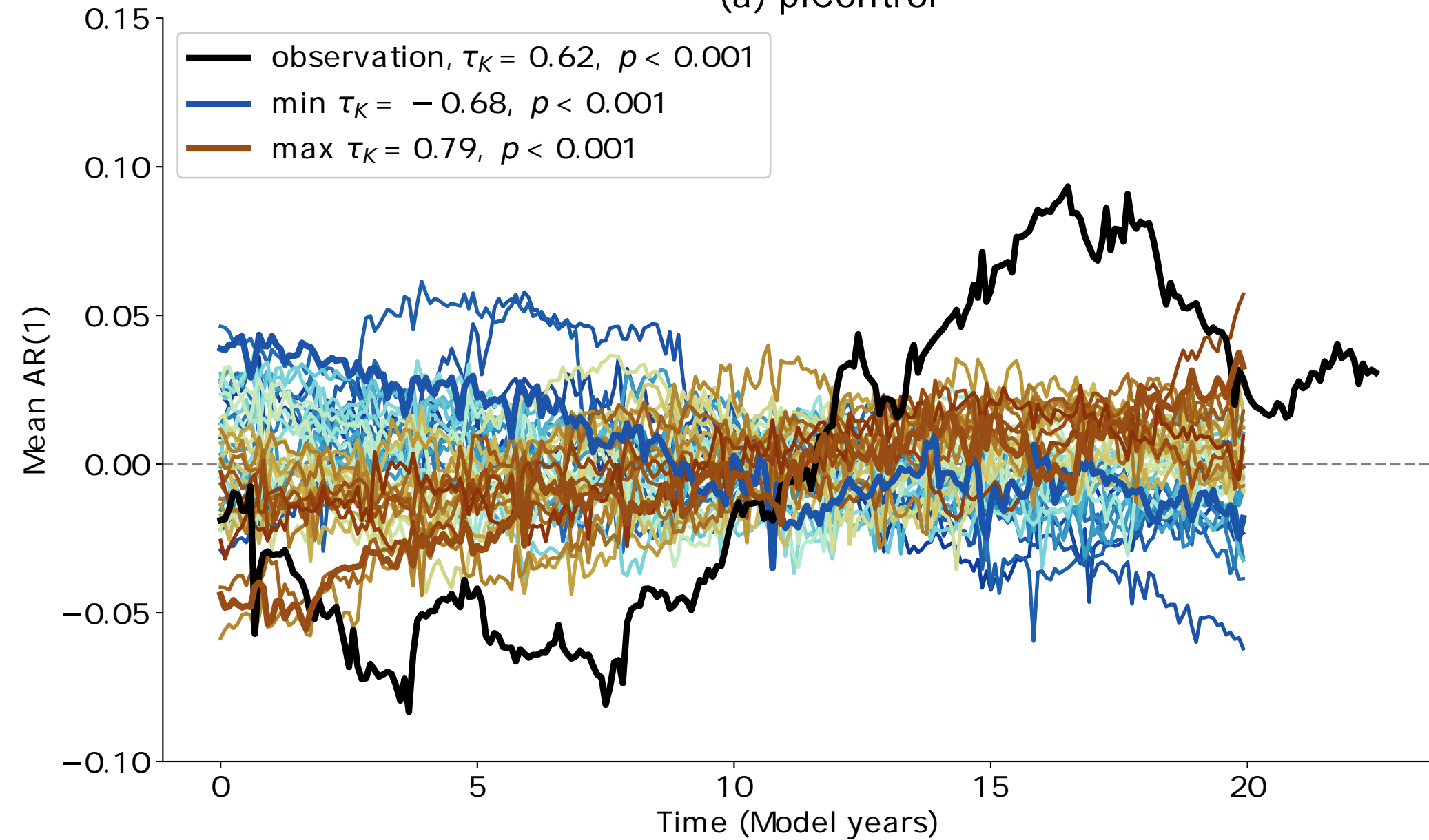
(a) piControl
