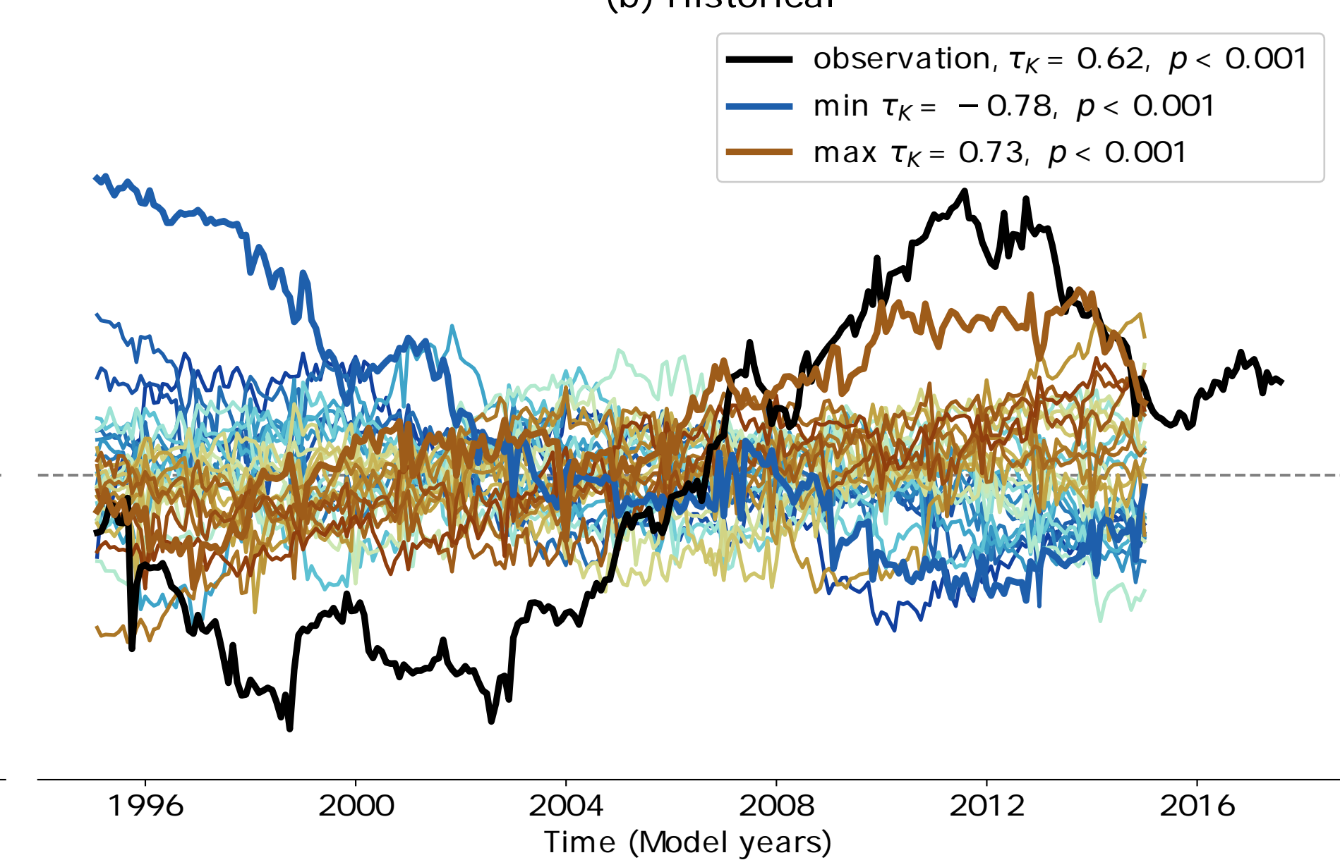
(b) Historical
