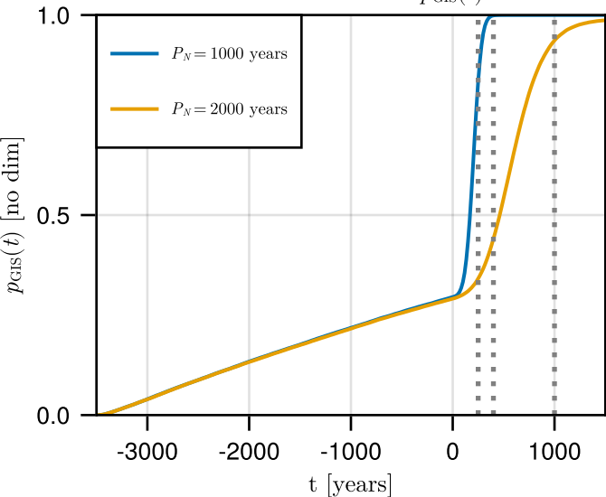
Time Evolution of p_{\text{GIS}}(t)
