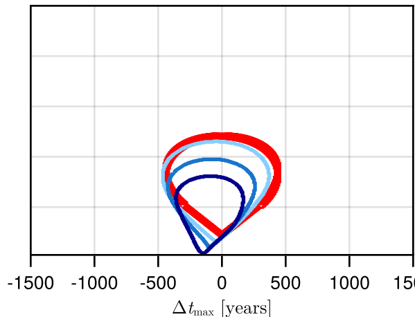
(b) In the (\Delta t_{\max}, P_S) parameter space
