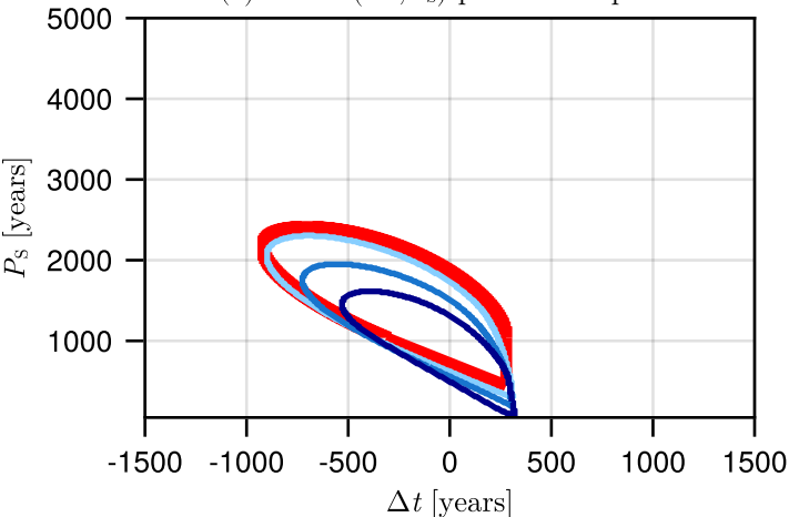
(a) In the (\Delta t, P_S) parameter space
