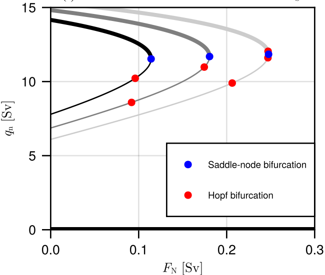
(a) Bifurcation Structure for Different F_S
