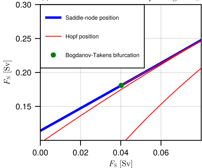
(b) Position of Bifurcations Depending on F_S
