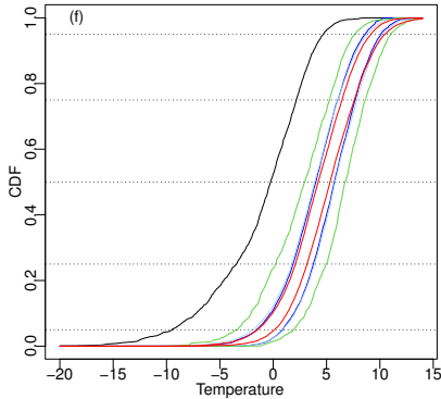
T, Stockholm, winter, 2081–2100
