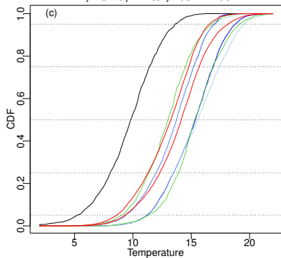
T, Berlin, winter, 2081–2100
