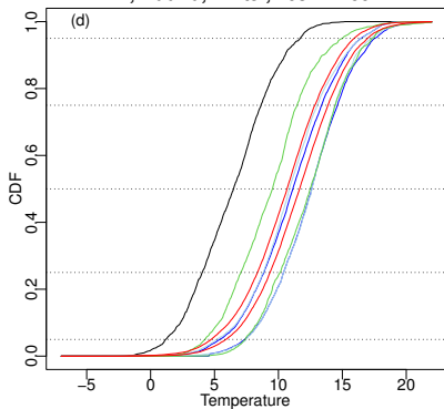
T, Stockholm, winter, 2081–2100
