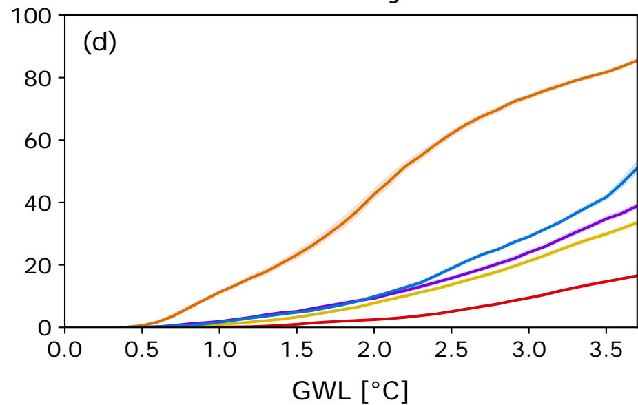
Rx1day
