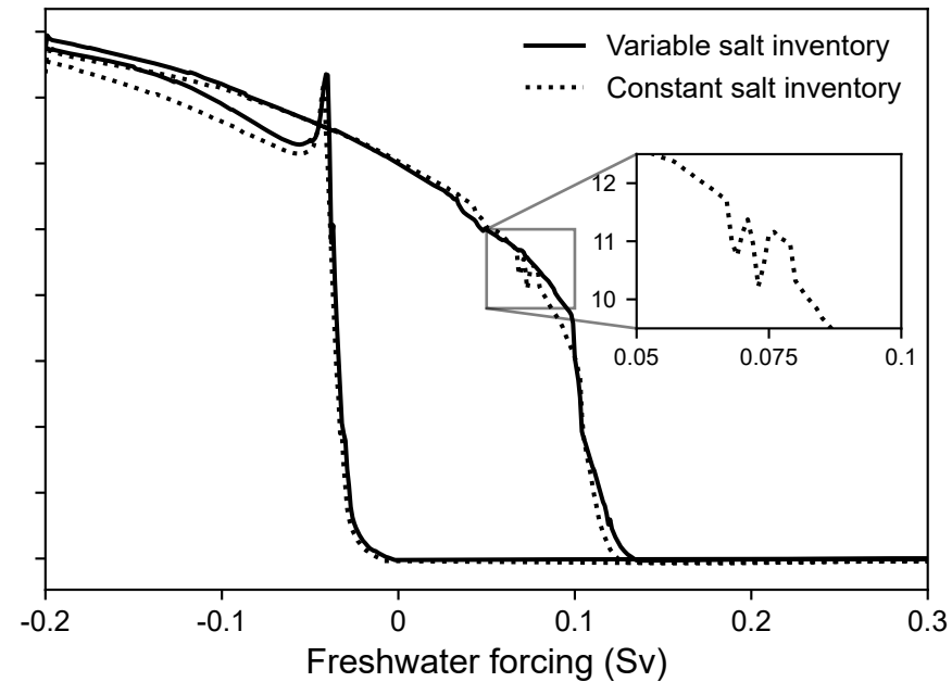
(b) AMOC hysteresis with freshwater
