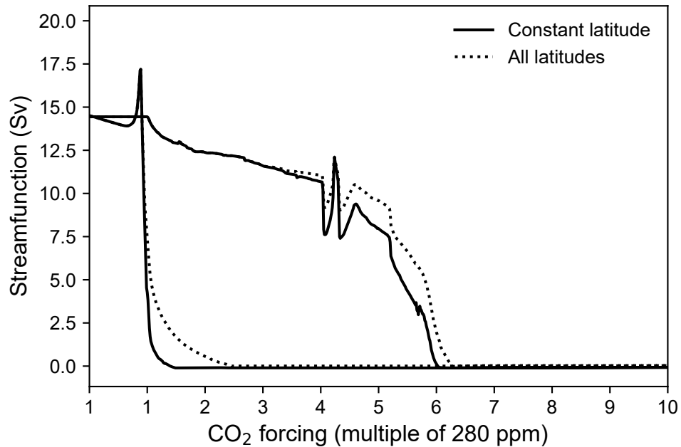
(a) AMOC hysteresis with CO 2
