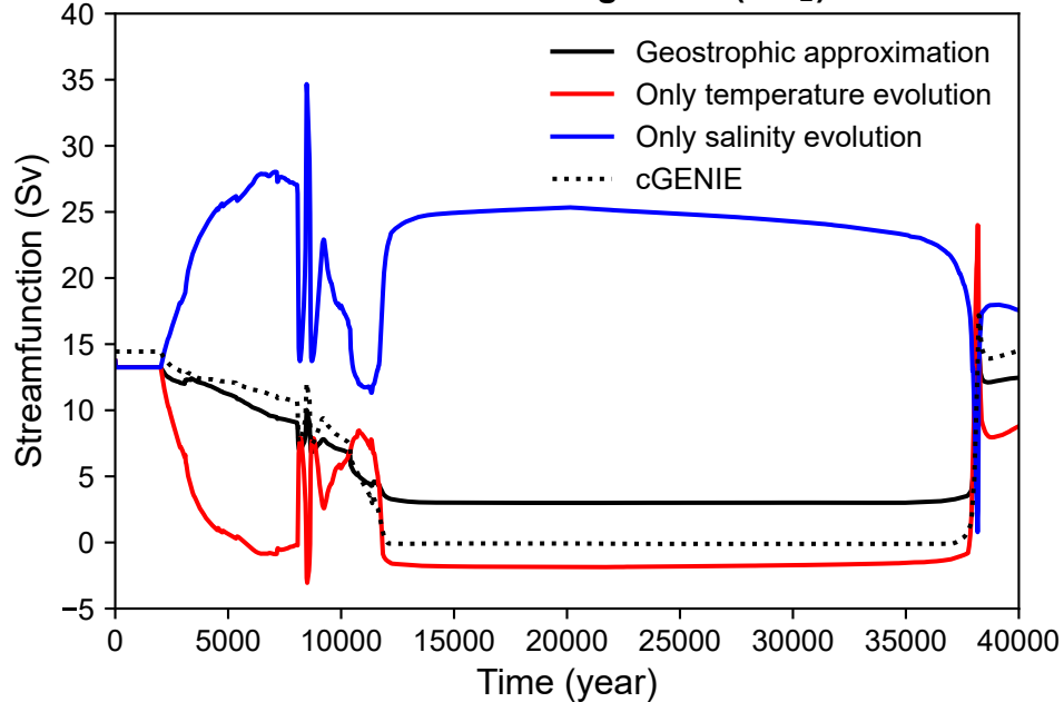
(c) Thermal wind diagnostic (CO 2 )
