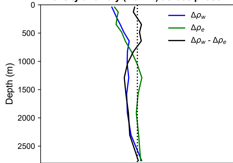
(a) Density anomaly (from T) across phase 1
