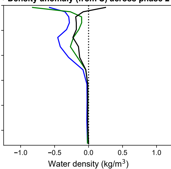
(e) Density anomaly (from S) across phase 2
