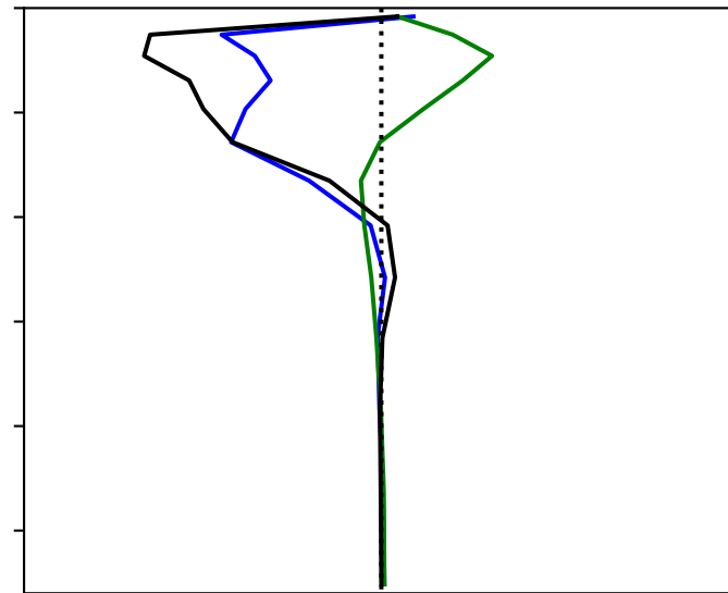
(c) Density anomaly (from T) across phase 3
