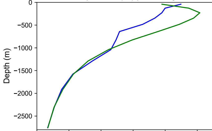
(e) Vertical temperature ( ^{\circ}\text{C} ) profile at year 2300
