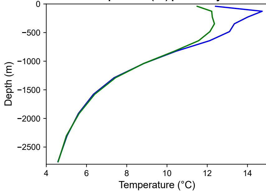
(g) Vertical temperature ( ^{\circ}\text{C} ) profile at year 3000
