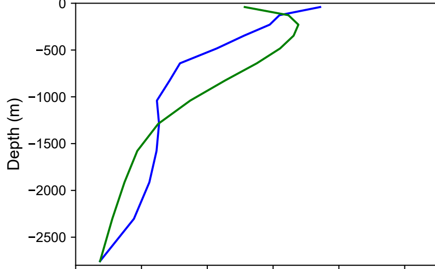
(c) Vertical temperature ( ^{\circ}\text{C} ) profile at year 2100
