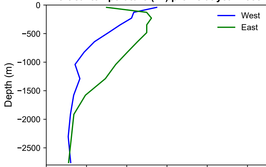
(a) Vertical temperature ( ^{\circ}\text{C} ) profile at year 2000
