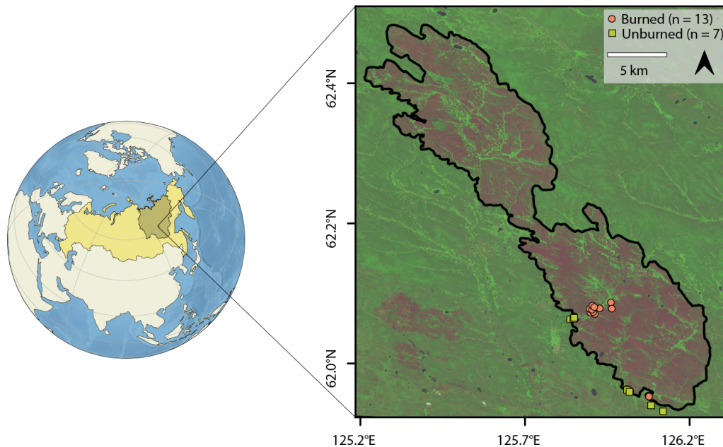
Figure 1. Map of the study area in the Republic of Sakha, Russia. The fire scar is shown in the reddish brown colors in a Landsat 8 Operational Land Imager false-color composite (RGB 754) from 23 July 2019. The locations of burned and unburned field plots are shown on the map.
