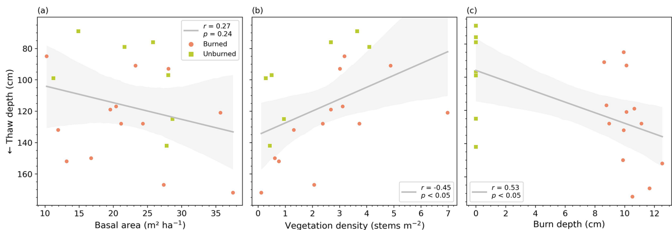
Figure 4. Relationships between field-measured thaw depth and (a) basal area, (b) vegetation density, and (c) burn depth. The shading around the regression lines indicates the 95 % confidence interval, while r is the Pearson correlation coefficient.
