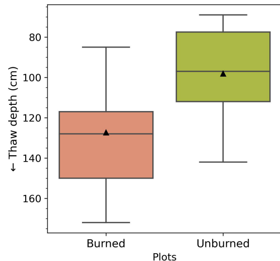
Figure 2. The 1-year post-fire summer thaw depth was deeper in burned plots compared to unburned plots. Each box ranges from the first to the third quartile. Whiskers extend to points that lie within 1.5 times the interquartile range. The median is indicated by the horizontal line and the mean by the black triangle.
