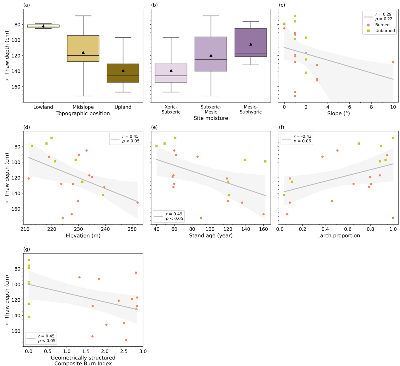
Figure B1. Relationships between thaw depth and (a) topographic position, (b) site moisture, (c) slope, (d) elevation, (e) stand age, (f) larch proportion, and (g) Geometrically structured Composite Burn Index. In (a) and (b), each box ranges from the first to the third quartile. Whiskers extend to points that lie within 1.5 times the interquartile range. The median is indicated by the horizontal line and the mean by the black triangle. For site moisture, classes were grouped together for better visualization. In the regression lines, shading indicates the 95 % confidence interval and r is the Pearson correlation coefficient.
