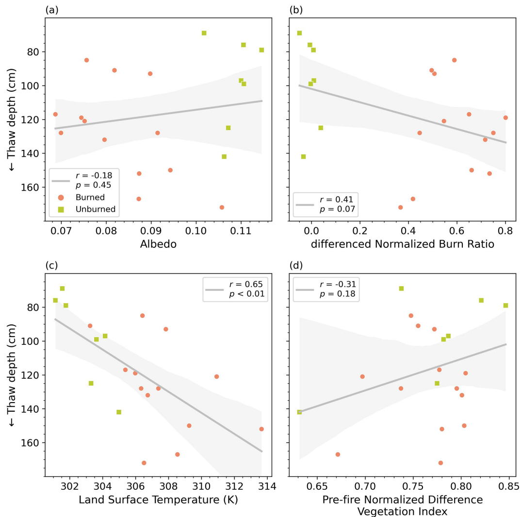
Figure 7. Scatter plots and linear regression lines between field-measured thaw depth and remotely sensed (a) albedo, (b) differenced normalized burn ratio, (c) land surface temperature, and (d) pre-fire normalized difference vegetation index. The shading indicates the 95 % confidence interval for the regressions and r is the Pearson correlation coefficient.
