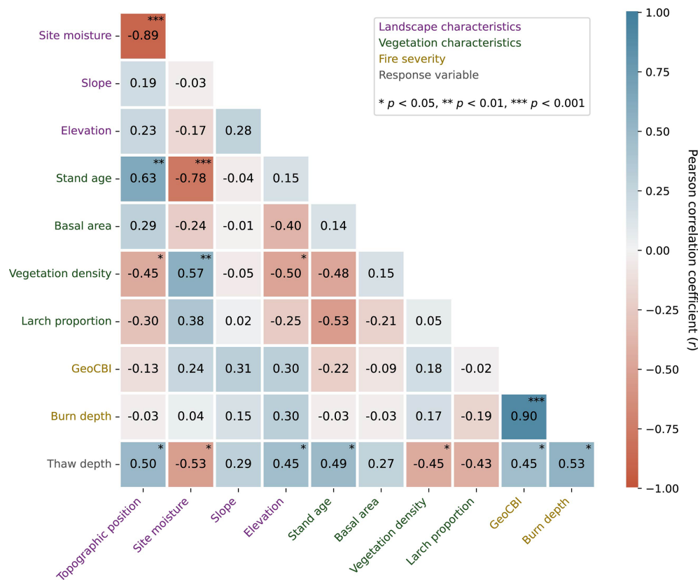
Figure 3. Correlation matrix between field-measured environmental variables representing landscape, vegetation and fire severity characteristics, and thaw depth. GeoCBI is the Geometrically structured Composite Burn Index.
