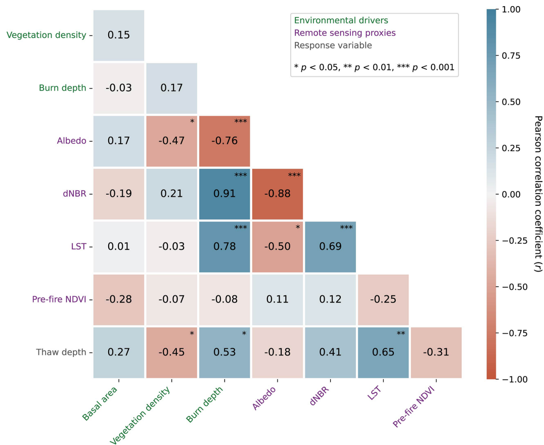
Figure C1. Correlation matrix of selected environmental drivers, remote sensing proxies, and thaw depth. GeoCBI is the Geometrically structured Composite Burn Index. LST is the land surface temperature. dNBR refers to the differenced normalized burn ratio and NDVI to the normalized difference vegetation index.
