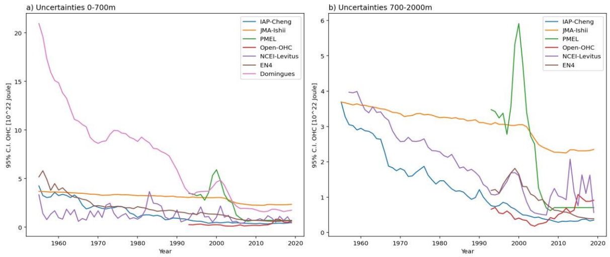
Figure S6: The uncertainties in the observational based series for OHC (Table A2). In a) for the upper 700 meters and in b) for 700 to 2000 meters.
