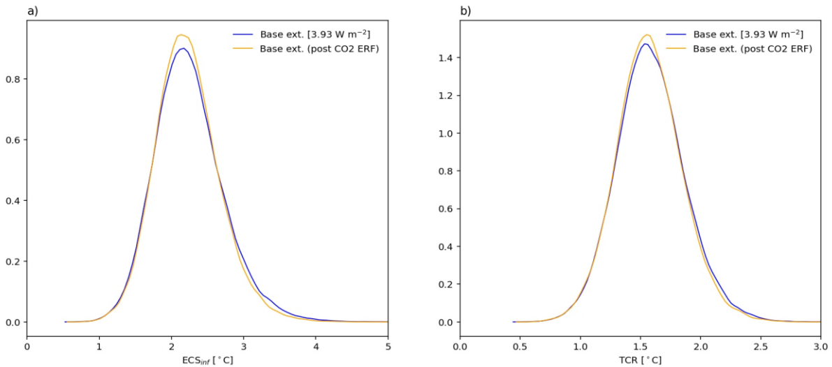
Figure S13: The ECS_{inf} (a) and TCR (b) probability density functions (PDF) for the “Base extended” using the best estimate of 2xCO_2 ERF from IPCC AR6 (blue) and the 2xCO_2 ERF corresponding to the posterior value of the CO_2 ERF in 2022 (orange). To get the 2xCO_2 ERF corresponding to the posterior value of CO_2 ERF, we scale the AR6 best estimate for 2xCO_2 of 3.93 \text{ W m}^{-2} (Forster et al., 2021) with the ratio of the posterior value for each ensemble member and the prior mean value for the CO_2 ERF for the end year. Similarly, we use the same scaling factor adjusting the ERF for 1% per year increase in CO_2 concentration used for the TCR calculation.
