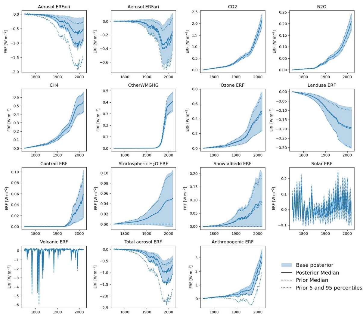
Figure S10: Prior and posterior distribution for the historical ERFs for all forcing components included in "Base". The prior median is shown as dashed line and the 5 th and 95 th percentile as dotted lines. The posterior median is shown as solid line and the 5 th to 95 th range as shading. In addition, the total aerosol ERF which is the sum of Aerosol ERFaci and Aerosol ERFari as well as the Anthropogenic ERF is shown.
