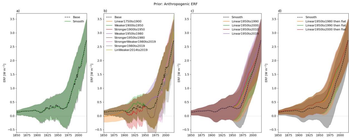
Figure S8: Same as Fig. S7 but for total anthropogenic ERF.
