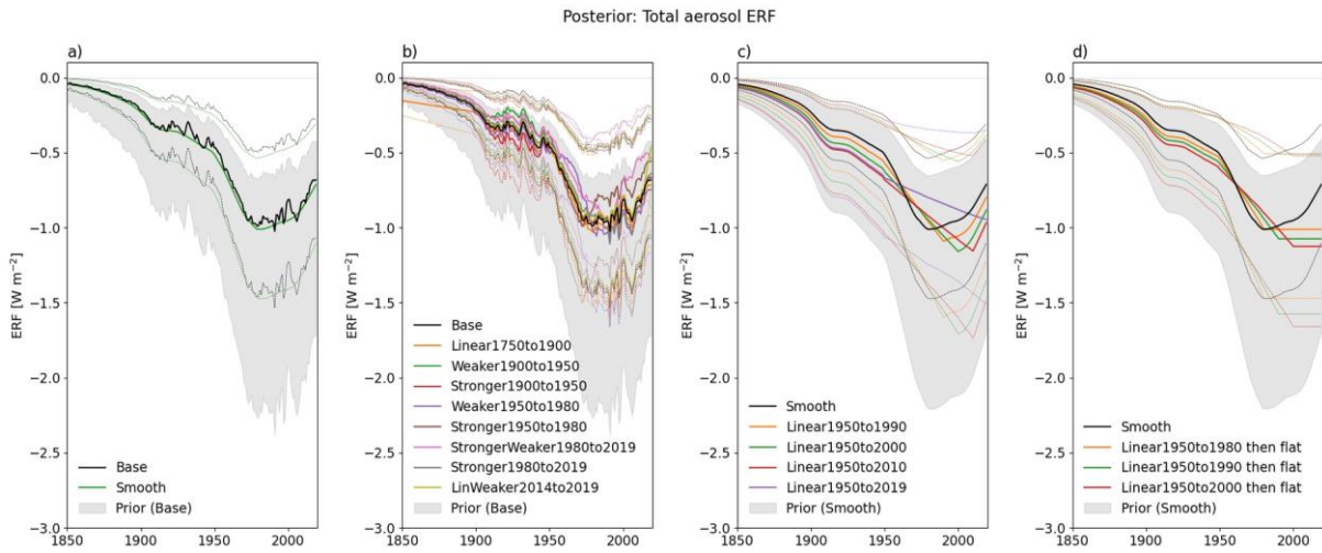
Figure S11: Posterior ERF time series for total aerosol ERF for the sensitivity tests. The mean value is indicated by a thick line and 90% C.I. by dashed lines. The gray shading indicate the 90% C.I. AR6 prior (in a,b) and the smoothed AR6 prior (in c,d) for reference. The priors for the individual tests are presented in Fig. S7.
