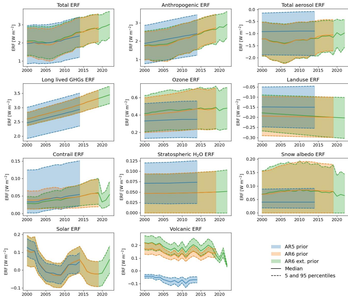
Figure S2: Same as Fig. S1, but ERF priors for a shorter period is shown.
