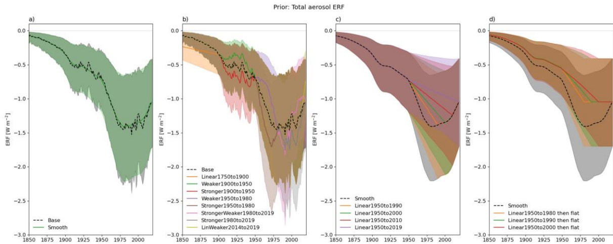
Figure S7: Prior total aerosol ERF time series for “Base” and for the aerosol ERF sensitivity tests. The mean value is indicated by a line and 90% uncertainty range by the shading. Both the ERF ari and ERF aci are adjusted in the sensitivity tests, and the sensitivity test are described in Table A3.
