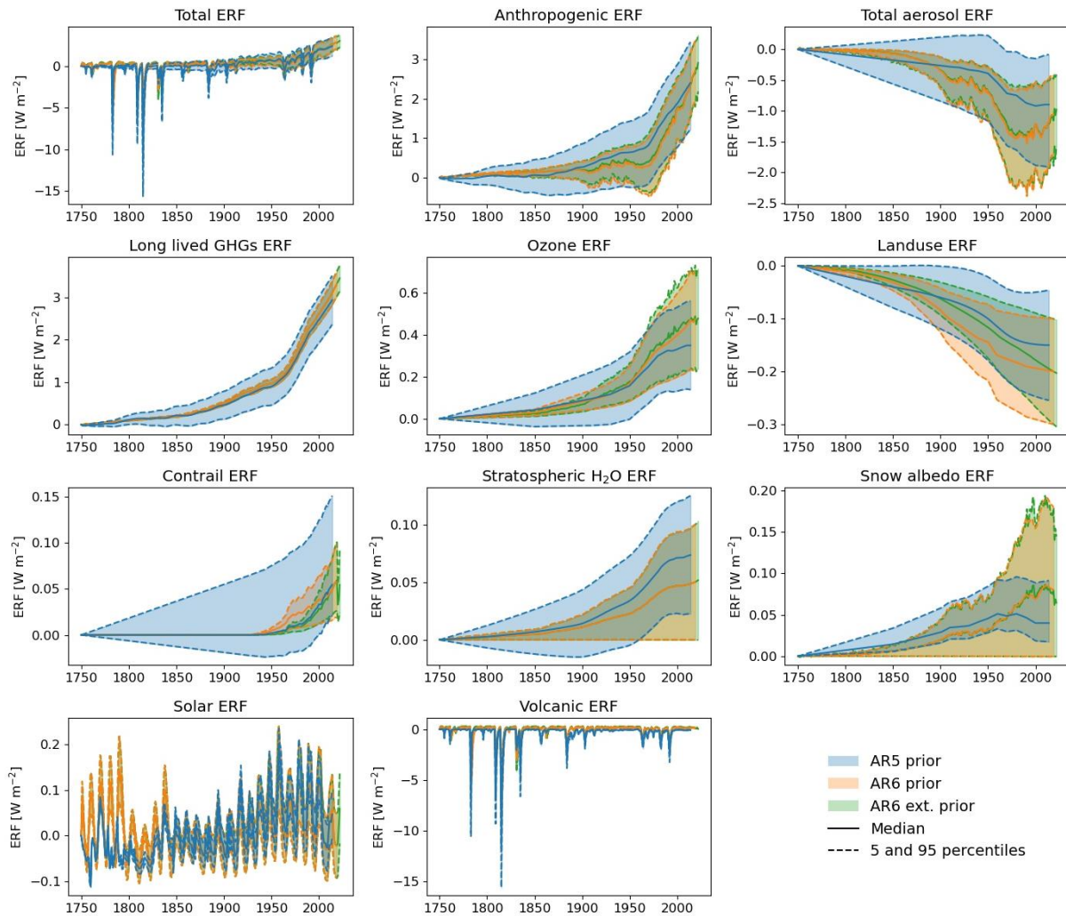
Figure S1: Prior ERF timeseries for the different forcing components. The shading and the dashed lines indicate the 90 % uncertainty ranges, and the solid line is the median ERF time series. Values from IPCC AR5 (Myhre et al., 2013) with historical uncertainty as implemented in Skeie et al. (2018) are shown in blue, from IPCC AR6 (Forster et al., 2021) in orange and IPCC AR6 extended to 2022 (Forster et al., 2023) in green. The components plotted here are the components included in IPCC AR5. For AR6 and AR6 extended the ERF for CO 2 , CH 4 , N 2 O and other well mixed greenhouse gases are used separately and the sum of these are shown here as Long lived GHGs. In AR6 and AR6 extended the total aerosol ERF are split between ERF ari and ERF faci but the sum is shown here for comparison with AR5. Note that the scale on y-axis differ and that uncertainties in contrail forcing was incorrectly implemented in Skeie et al. (2018) as ERF should have been zero before 1930.
