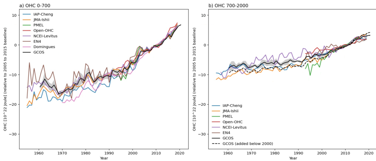
Figure S4: The observational based series for OHC used in “Base” as listed in Table A2. OHC anomalies (relative to reference period 2005 to 2015) for upper 700 meter in a) and 700 meters to 2000 meters in b). GCOS data from von Schuckmann et al. (2023) is added to the figure. The dashed black line in b) is GCOS data below 700 meters that includes OHC below 2000 meters.
