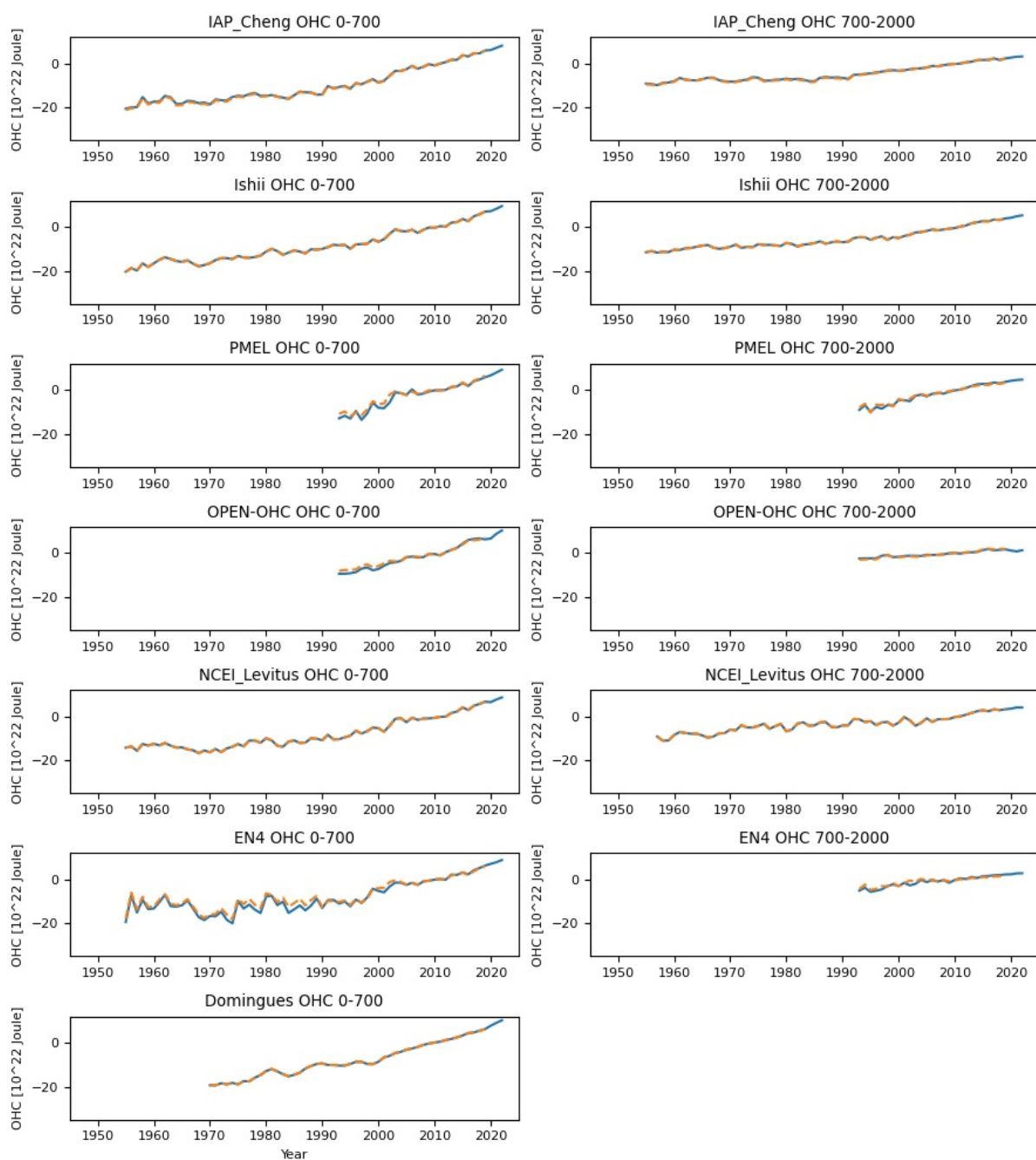
Figure S5: Anomalies for observed ocean heat content. OHC 0-700 meters (left) and OHC 700-2000 meters (right) for the different time series (Table A2). The blue lines are the updated data up to 2022 used in “Base extended” while the dashed orange lines are the data up to 2019 used in “Base”. The OHC data are plotted relative to a 2005 to 2015 baseline.
