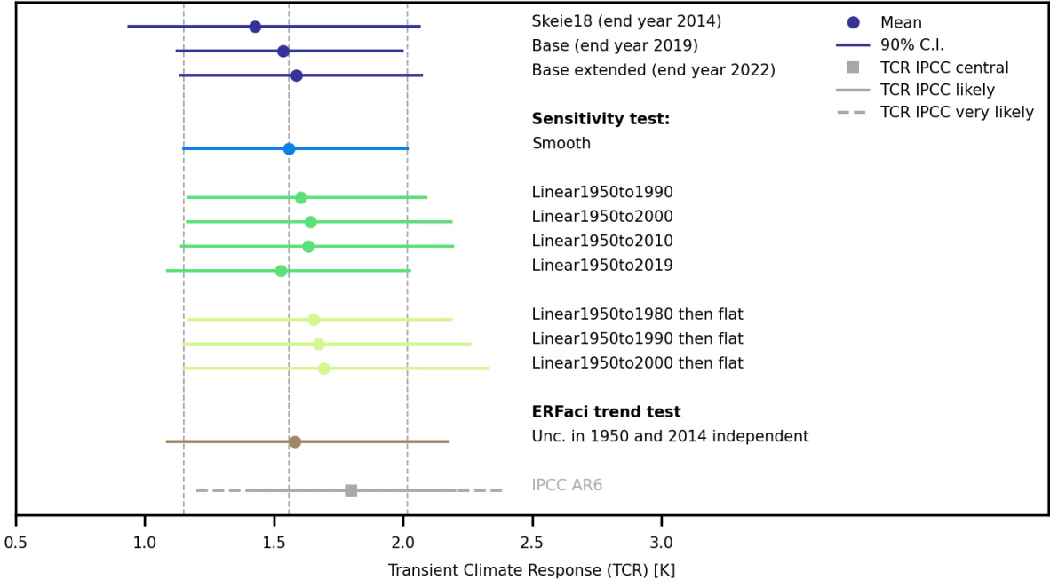
Figure S9: Posterior Transient Climate Response (TCR) for the different analyses and sensitivity tests. The 90% C.I. is indicated by a solid line and the mean values as a dot. The vertical lines indicate the posterior mean value and 90% C.I. for “Smooth”, as it is used as a starting point for the “Linear” sensitivity tests shown. The TCR central estimate, and likely (66% probability) and very likely (90% probability) ranges from IPCC AR6 (Forster et al., 2021) are shown in grey colours at the bottom. The posterior mean, median and 5 and 95 percentiles are presented in Table S2.
