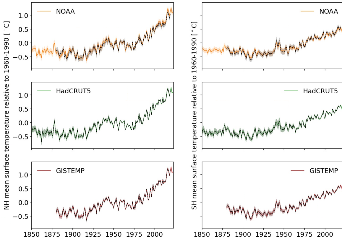
Figure S3. Hemispheric annual mean surface temperature for the three different observational based series (Table A2) used in the estimation. Temperatures are plotted relative to a 1960-1990 baseline and the shading indicates uncertainty of one standard deviation. The colored lines are the updated values to 2022 used in “ Base extended ”, while the black dashed lines are the values up to 2019 used in “ Base ”.
