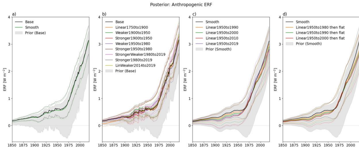
Figure S12: Same as Fig. S11, but for total anthropogenic ERF. The prior for the individual tests are presented in Fig. S8.
