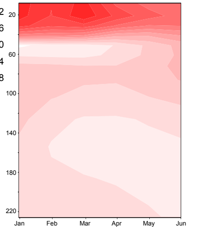
(e) ROM F - ROM P
