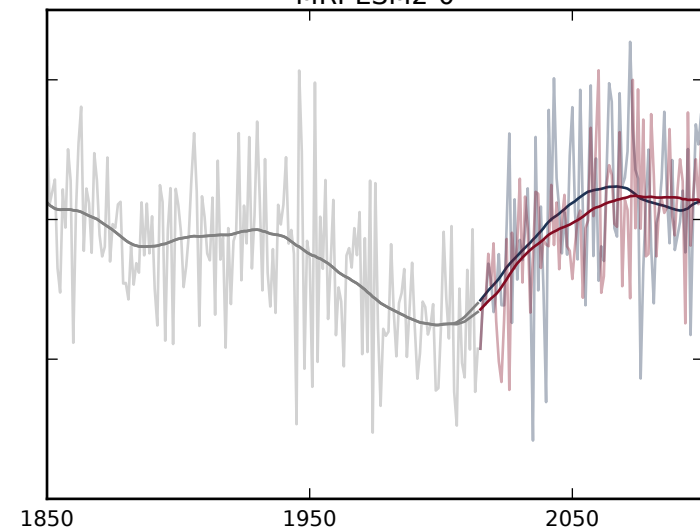
MRI-ESM2-0
