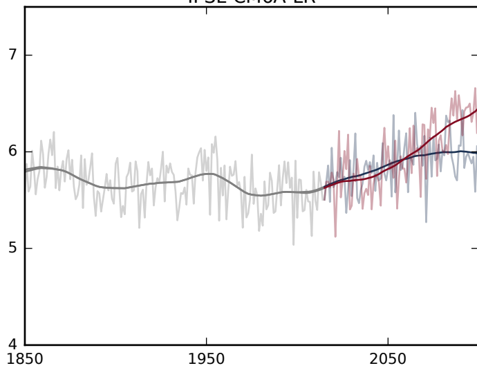
IPSL-CM6A-LR
