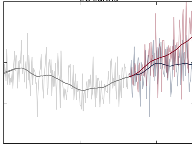
EC-Earth3
