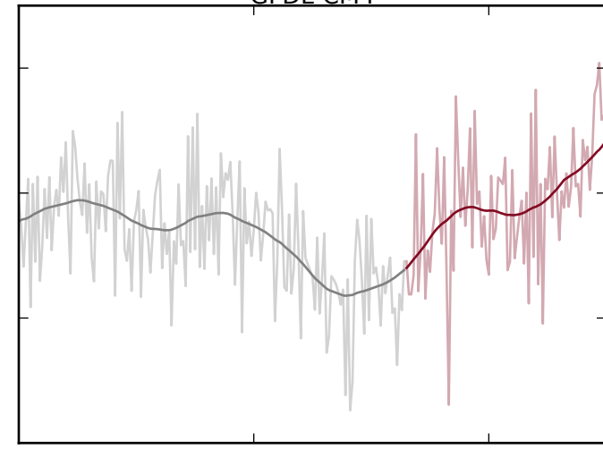
GFDL-CM4
