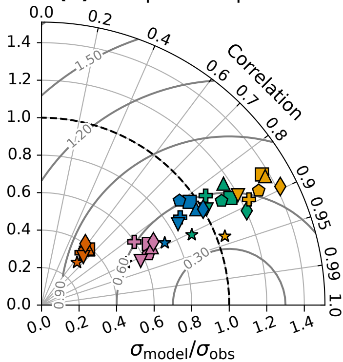
(a) GPP peak amplitude
