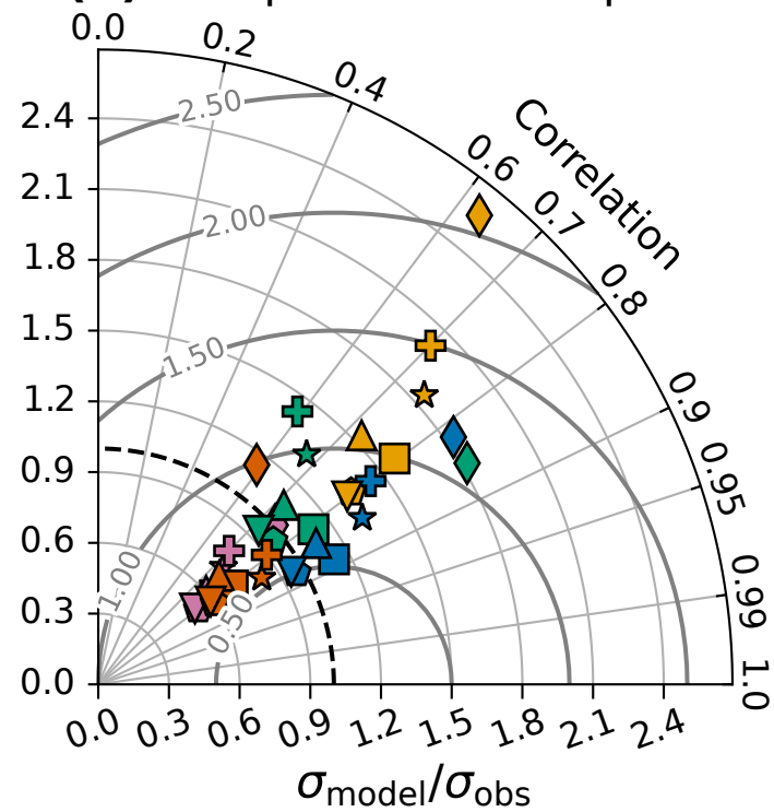
(b) GPP post-event amplitude
