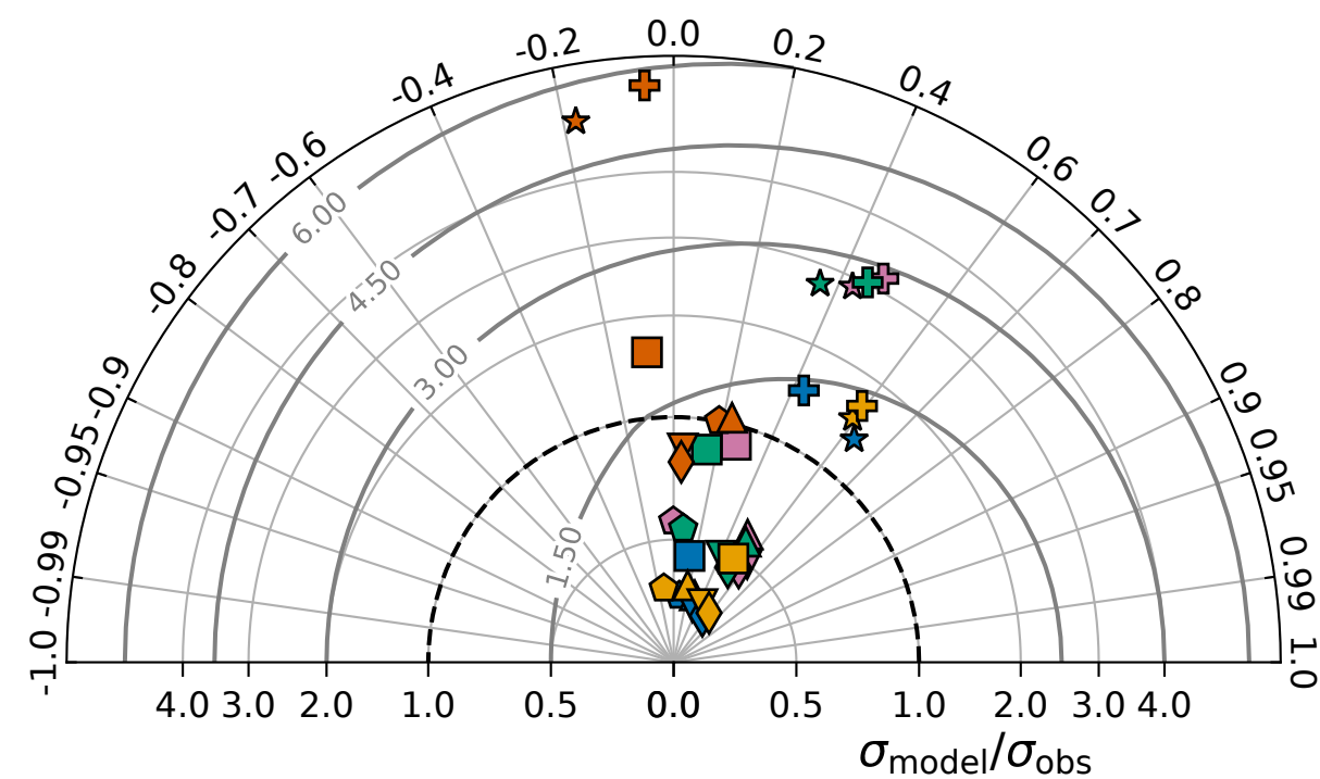
(c) GPP lag
