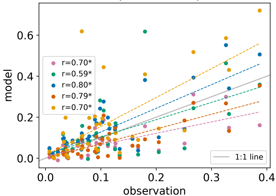
(c) GPP post-event amplitude
