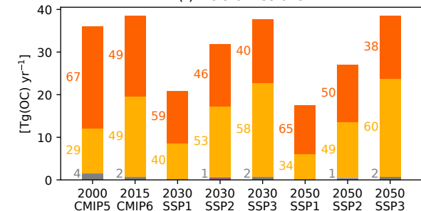
(f) - OC emissions
