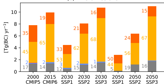
(e) - BC emissions
