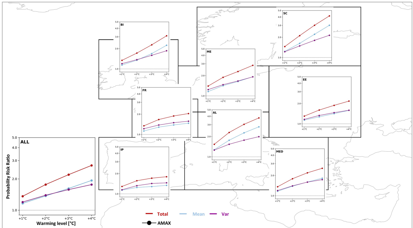
Figure 4. Regional averaged PR values (total, mean, and var) for the PRUDENCE regions at different warming levels for annual rx3h (AMAX) events larger than 2\sigma . PR_{total} (red), PR_{mean} (blue), and PR_{var} (purple) values (y axis) at warming levels (+1, +2, +3, +4 °C) (x axis). The lower-left panel (ALL) shows the aggregation over all land grid cells and shows axis labels that apply for all panels.
