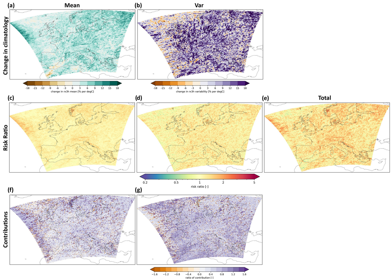
Figure 2. Changes in the current climate (+1 °C) compared to a stable pre-industrial climate in the CRCM5-LE simulations. (a) Change in the mean annual rx3h. (b) Change in the variability (i.e., standard deviation of annual rx3h). (c) PR_{\text{mean}} , (d) PR_{\text{var}} , and (e) PR_{\text{total}} values for 2\sigma events. (f) Ratio of contribution for changes in the mean. (g) Ratio of contribution for changes in variability.
