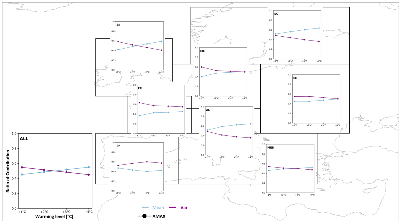
Figure 5. Individual contributions from PR_{\text{mean}} and PR_{\text{var}} to the PR_{\text{total}} in the different PRUDENCE regions at different warming levels. Ratio of contributions from PR values in Fig. 4. Contribution from the mean are shown in blue, and contributions from variability are shown in purple. Ratio of contribution is on the y axis, and different warming levels are on the x axis. The warming levels are +1, +2, +3, +4 °C. The lower-left panel (ALL) shows the aggregation over all land grid cells and shows axis labels that apply for all panels.
