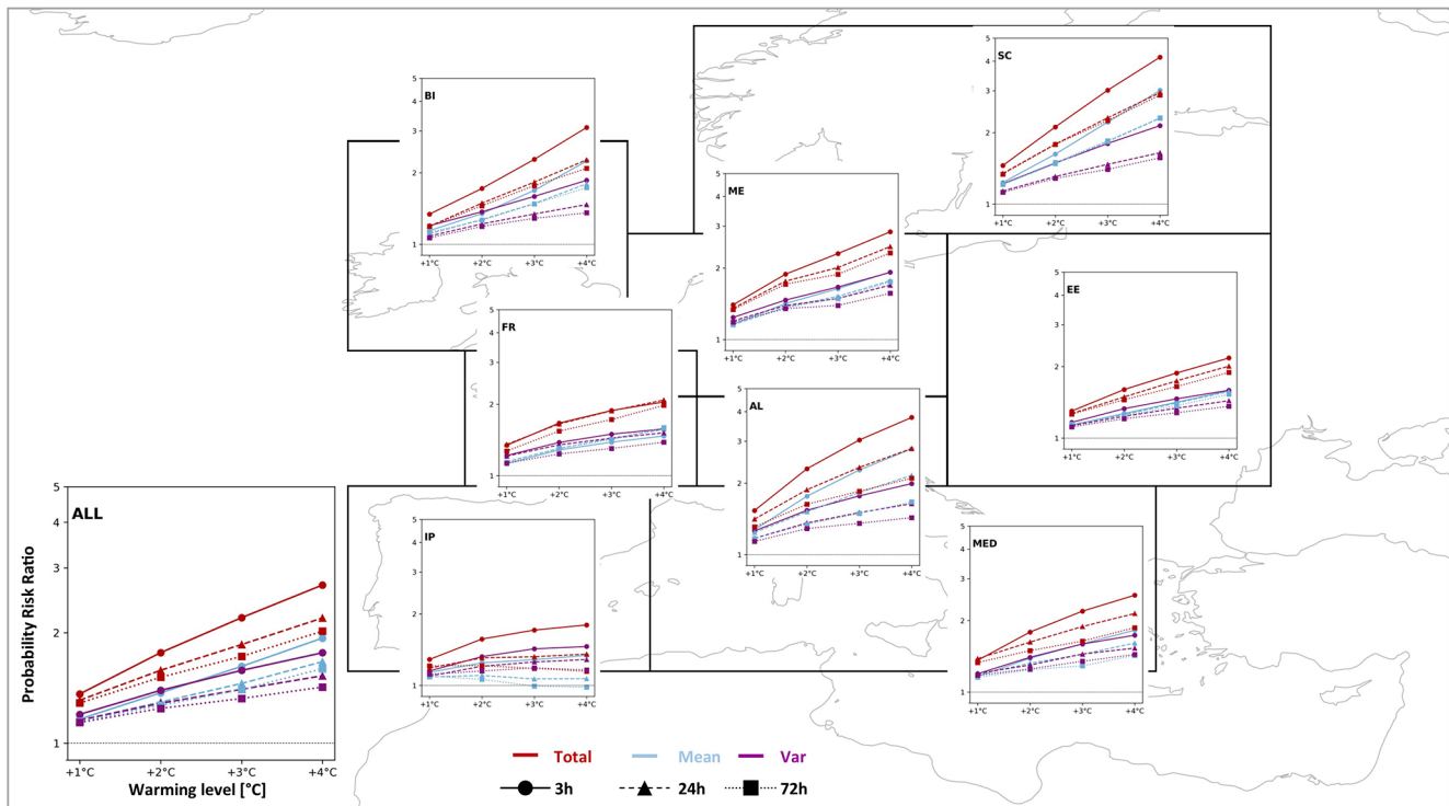
Figure 9. Regional probability risk ratios for different temporal aggregation levels (3, 24, 72 h) on annual scales. The panels show PR_{total} (red), PR_{mean} (blue), and PR_{var} (purple) values (y axis) at warming levels of +1, +2, +3, +4 °C (x axis). The solid lines with the circle marker represent PR values for 3 h temporal aggregation (the same as in Fig. 4); the dashed lines with the triangle marker represent PR values for 24 h; and the dotted lines with the square marker represent PR values for 72 h. The lower-left panel (ALL) shows the aggregation over all land grid cells and shows axis labels that apply for all panels.
