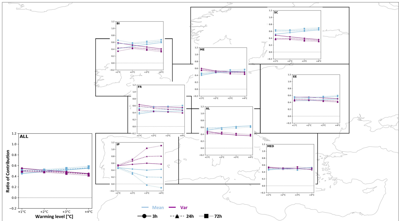
Figure 10. Regional ratios of contribution based on different levels of temporal aggregation (3, 24, and 72 h) for annual maxima. Ratio of contributions from PR values in Fig. 9. Contribution from the mean is shown in blue, and contributions from variability are shown in purple. Ratio of contribution is shown on the y axis, with different warming levels shown on the x axis (+1, +2, +3, +4 °C). The solid lines with the circle marker represent individual contributions for 3 h temporal aggregation (same as in Fig. 5); the dashed lines with the triangle marker represent contributions for 24 h; and the dotted lines with the square marker represent contributions for 72 h. The lower-left panel (ALL) shows the aggregation over all land grid cells and shows axis labels that apply to all panels.
