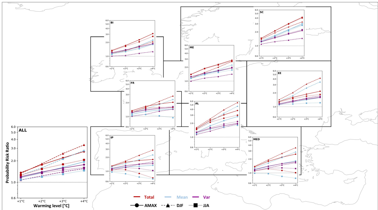
Figure 7. Comparison of regional averaged annual and seasonal PR values (total, mean, and var) at different warming levels. The panels show PR_{total} (red), PR_{mean} (blue), and PR_{var} (purple) values (y axis) at warming levels of +1, +2, +3, +4 °C (x axis). The solid lines with the circle marker represent annual PR values (AMAX, the same as in Fig. 4); the dashed lines with the triangle marker represent PR values in winter (DJF); and the dotted lines with the square marker represent PR values in summer (JJA). The lower-left panel (ALL) shows the aggregation over all land grid cells and shows axis labels that apply for all panels.
