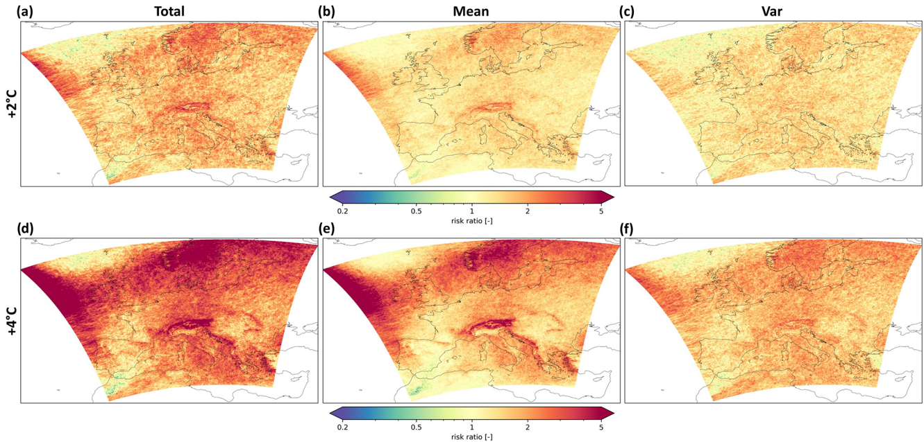
Figure 3. Probability risk ratios for annual rx3h for extreme events larger than 2\sigma in a 2 and 4 °C warmer world: (a, d) PR_{total} , (b, e) PR_{mean} , and (c, f) PR_{var} . Panels (a)–(c) show +2 °C climate, and panels (d)–(f) show +4 °C climate. All probabilities are relative to the pre-industrial climate.
