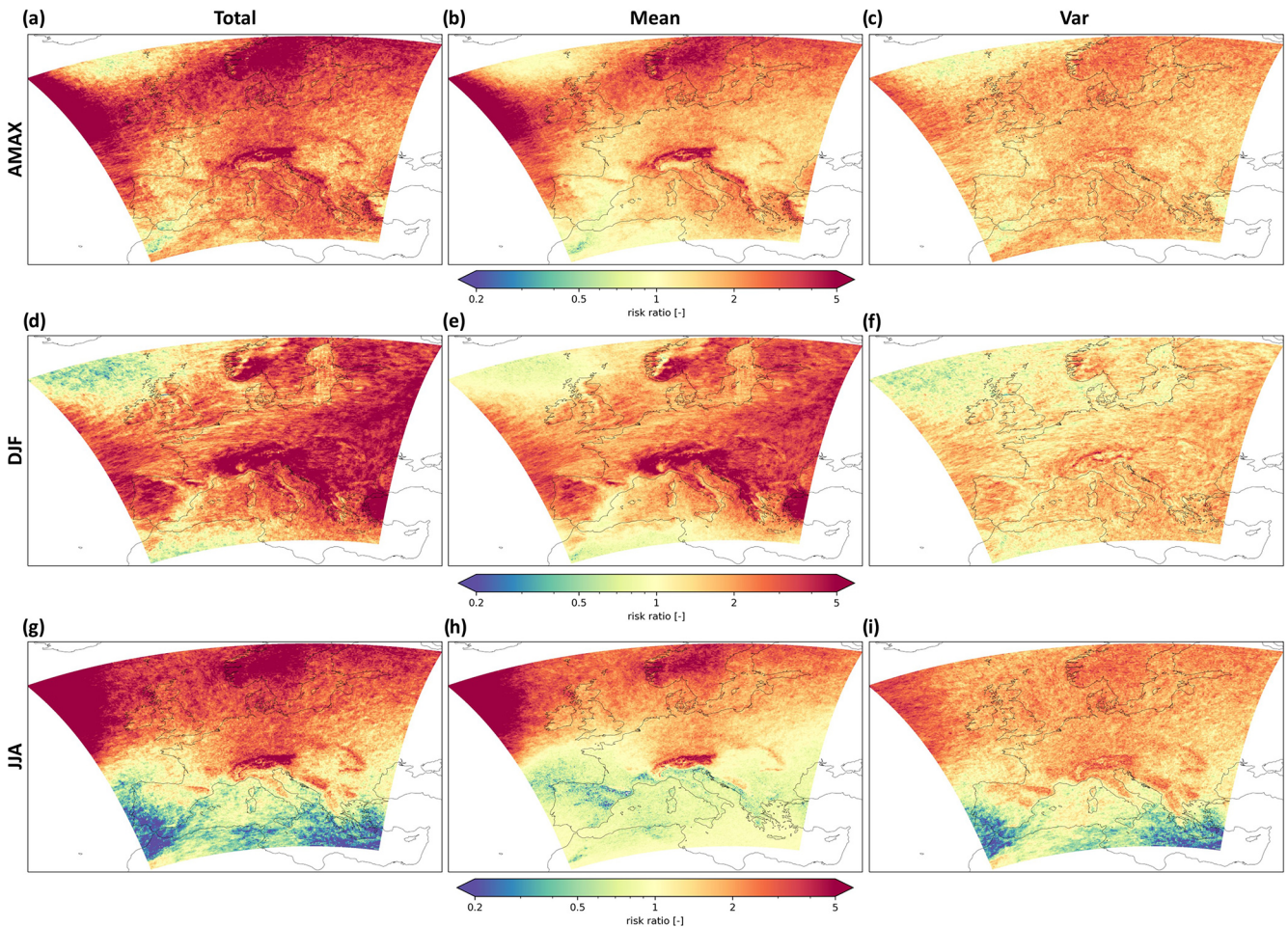
Figure 6. Annual probability risk ratios of rx3h events compared to seasonal DJF and JJA PR values at 4 °C warming: (a–c) annual PR values, (d–f) DJF PR values, (g–i) JJA PR values, (a, d, g) PR_{\text{total}} , (b, e, h) PR_{\text{mean}} , and (c, f, i) PR_{\text{var}} .
