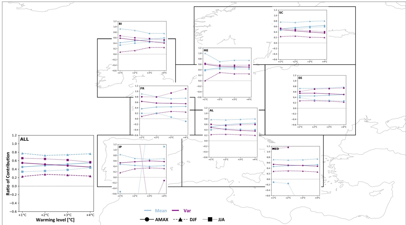
Figure 8. Comparison of individual contributions of annual and seasonal PR_{\text{mean}} and PR_{\text{var}} to the PR_{\text{total}} at different warming levels. Ratio of contributions from PR values in Fig. 7. Contribution from the mean are shown in blue, and contributions from variability are shown in purple. Ratio of contribution is shown on the y axis, with different warming levels shown on the x axis (+1, +2, +3, +4 °C). The solid lines with the circle marker represent annual ratio of contributions (AMAX, the same as in Fig. 5); the dashed lines with the triangle marker represent ratios in winter (DJF); and the dotted lines with the square marker represent ratios in summer (JJA). The lower-left panel (ALL) shows the aggregation over all land grid cells and shows axis labels that apply for all panels.
