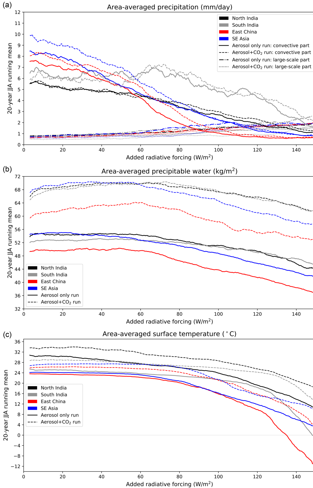
Figure 9. Precipitation (a), precipitable water (b), and surface temperature (c), averaged over the regions indicated (following the marked boxes in Fig. 5), for aerosol-only and aerosol-with-2 × CO 2 runs, against the absorbing aerosol forcing. Precipitation is separated into convective and large-scale components. Variables are taken as a running 20-year June–July–August mean.
