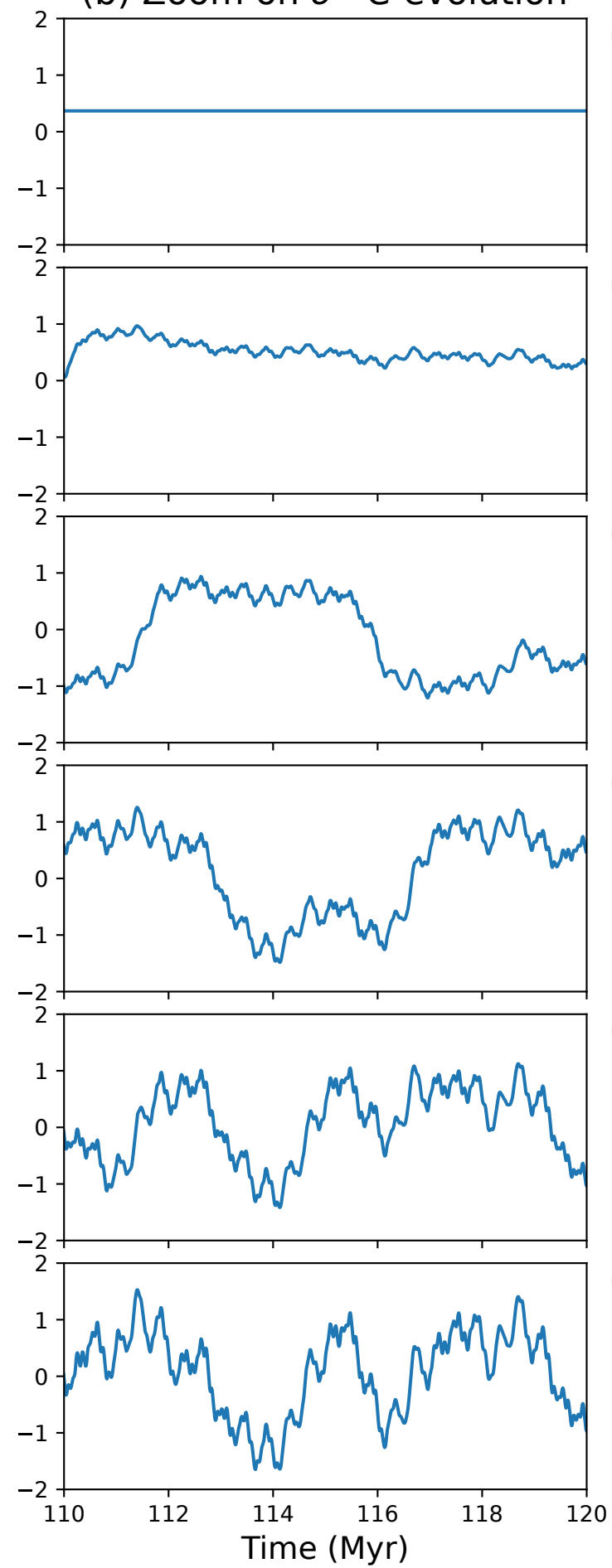
(b) Zoom on \delta^{13}\text{C} evolution
