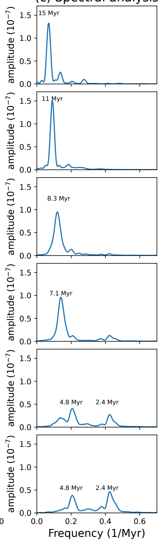
(c) Spectral analysis
