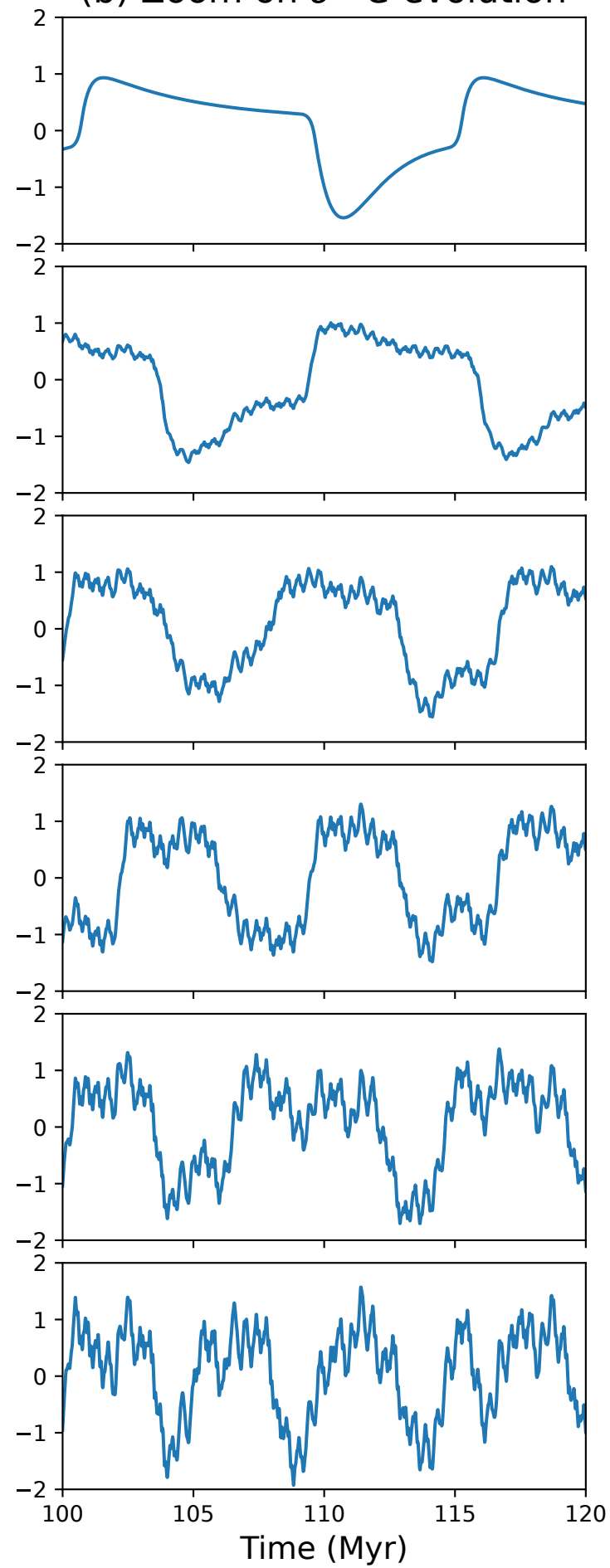
(b) Zoom on \delta^{13}\text{C} evolution
