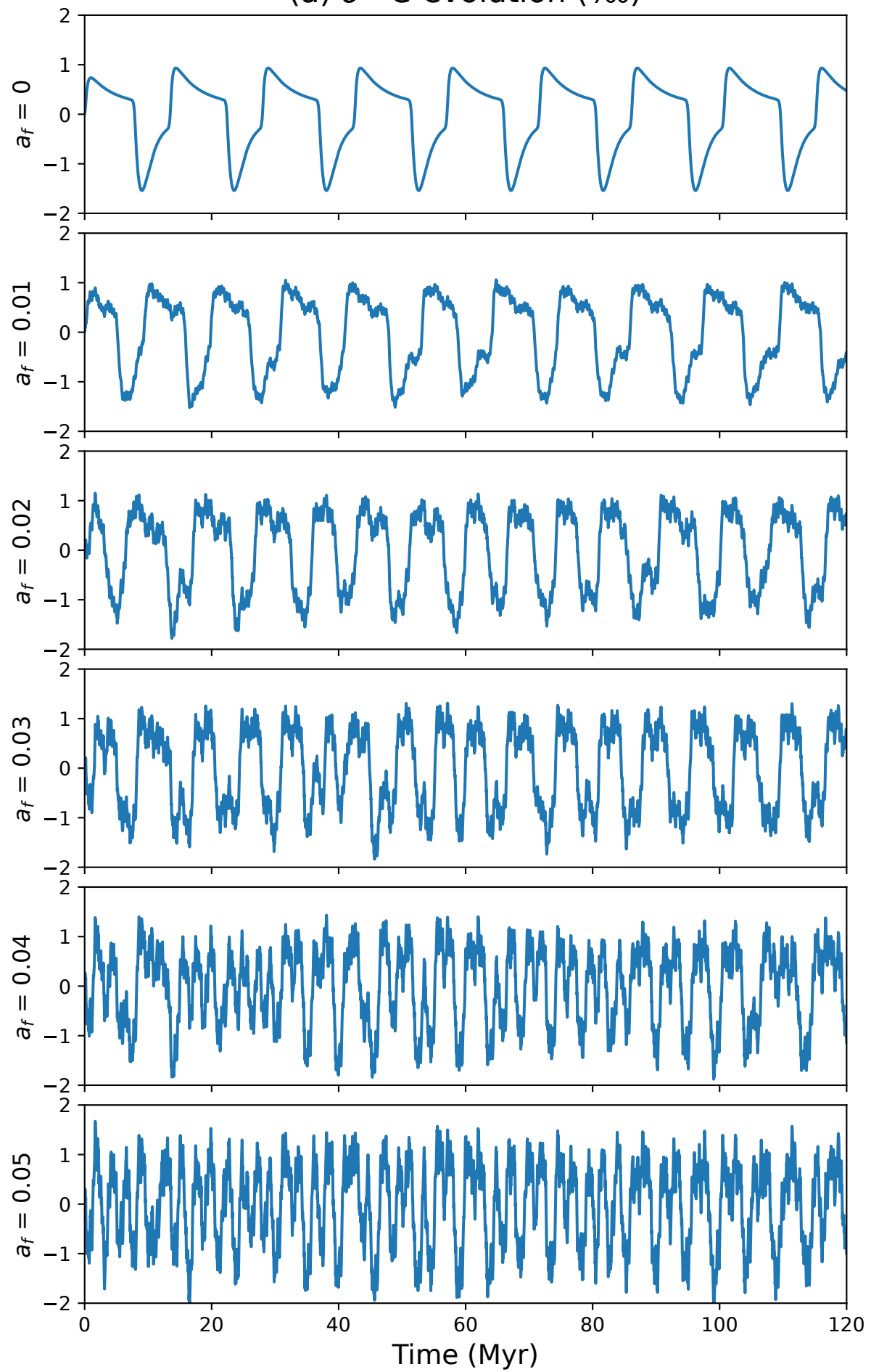
(a) \delta^{13}\text{C} evolution (‰)
