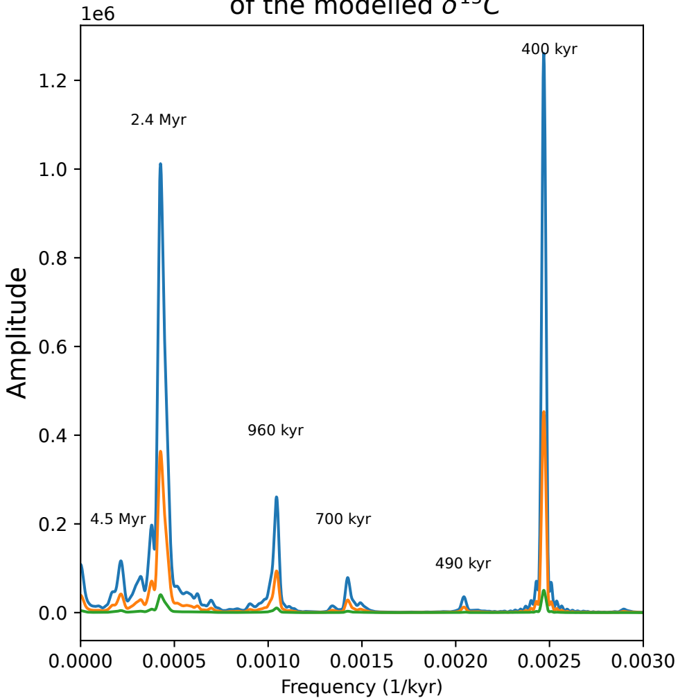
(a) Spectral analysis of the modelled \delta^{13}\text{C}
