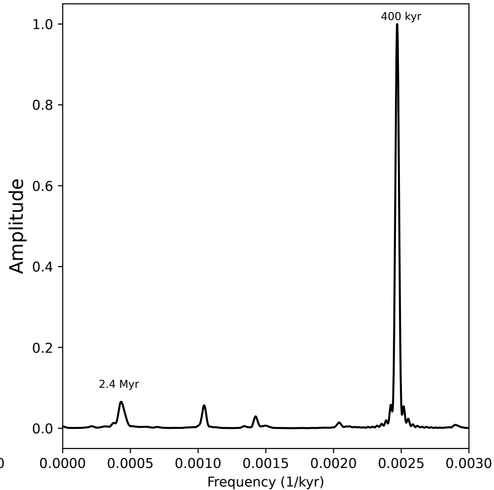
(b) Spectral analysis of eccentricity
