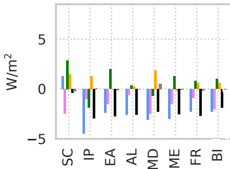
(c) DLR JJA
