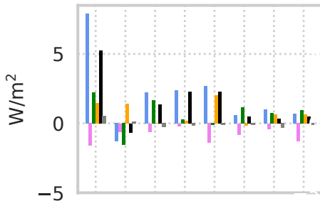
(c) DLR JJA
