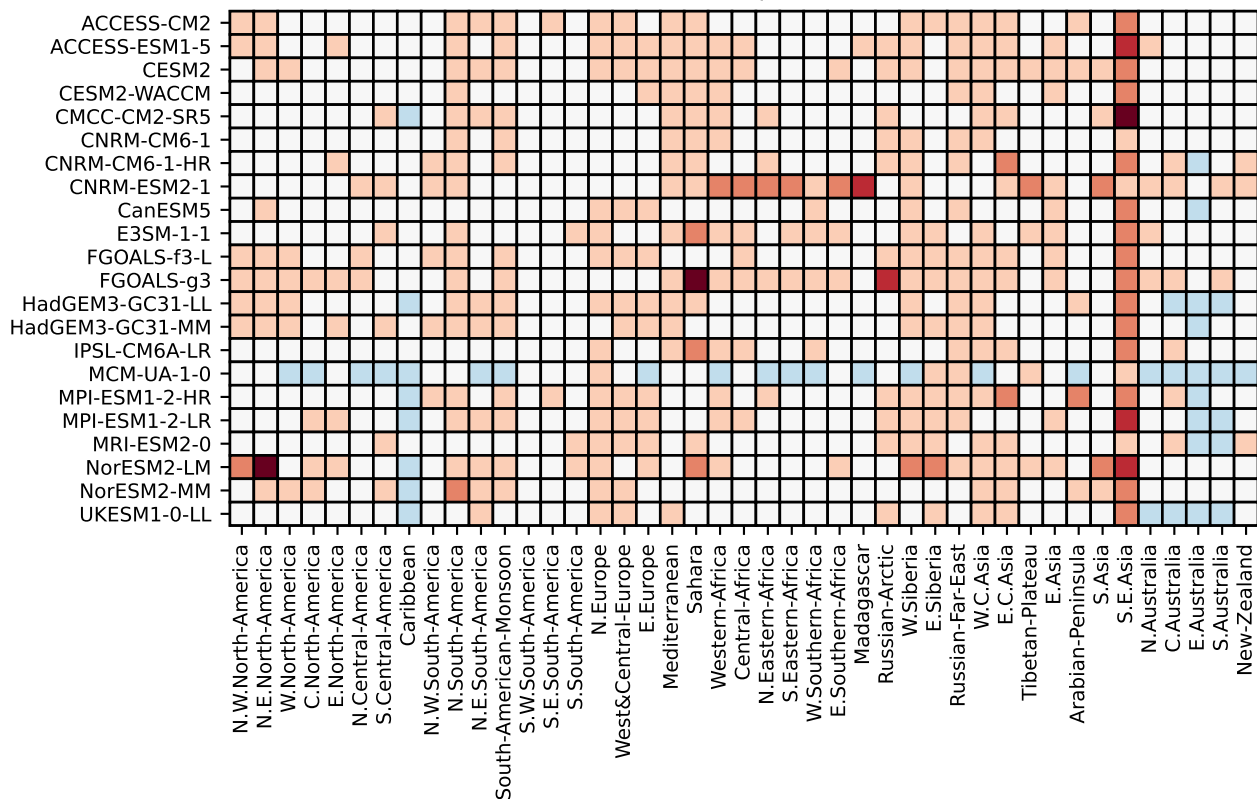
(c) 2.5% quantile
