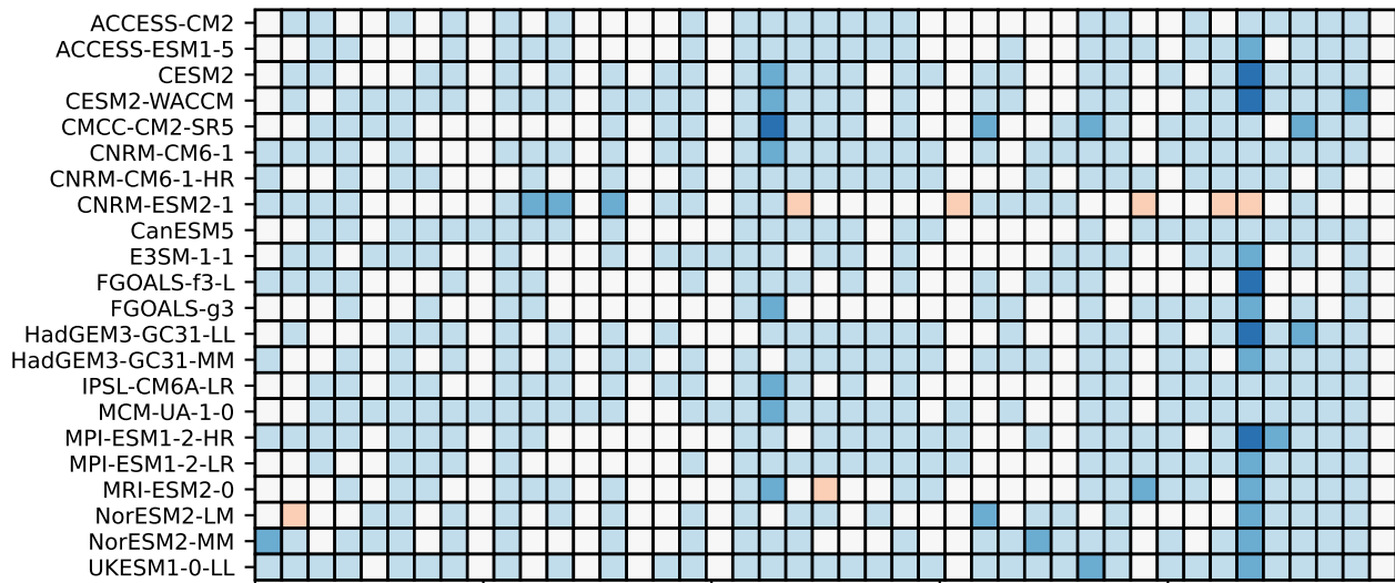
(a) 97.5% quantile
