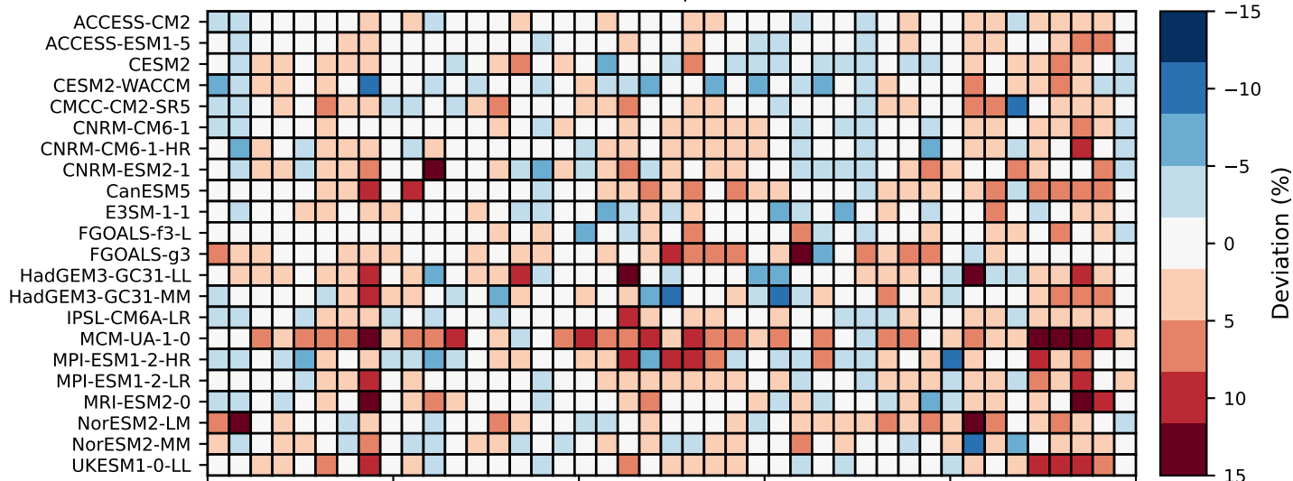
(c) 2.5% quantile
