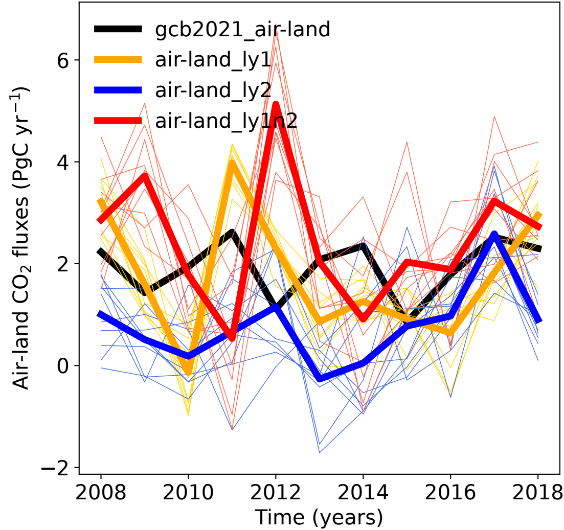
(b) Air-land CO 2 fluxes
