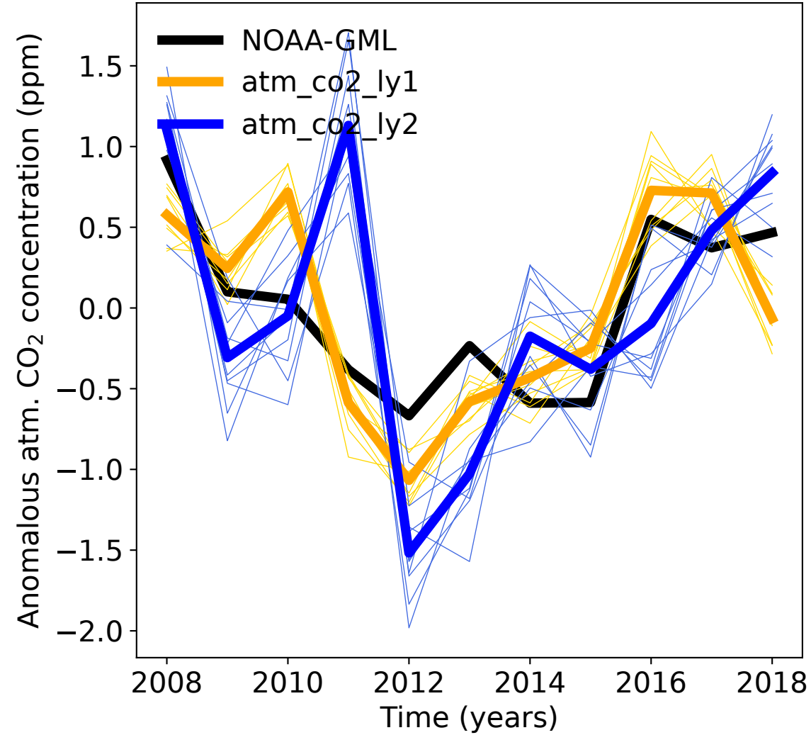
(a) Atmospheric CO 2 concentration
