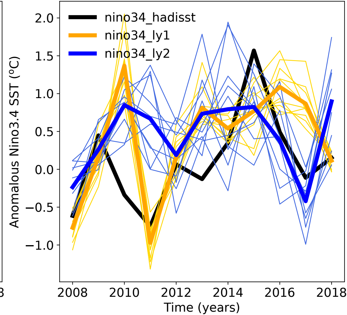
(c) Nino3.4 SST
