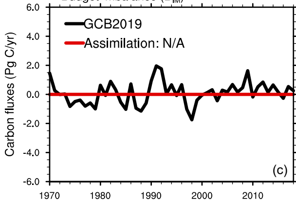
Budget imbalance ( B_{IM} )
