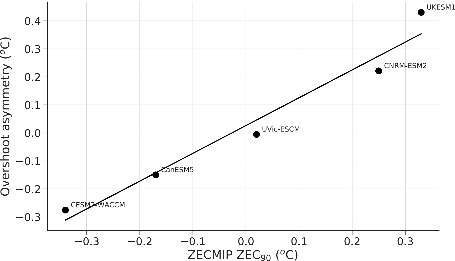
SSP5-3.4-overshoot temperature asymmetry versus ZECMIP ZEC 90
