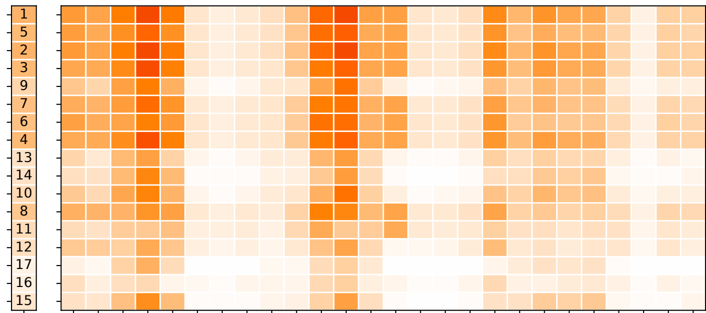
UKESM1-0-LL
