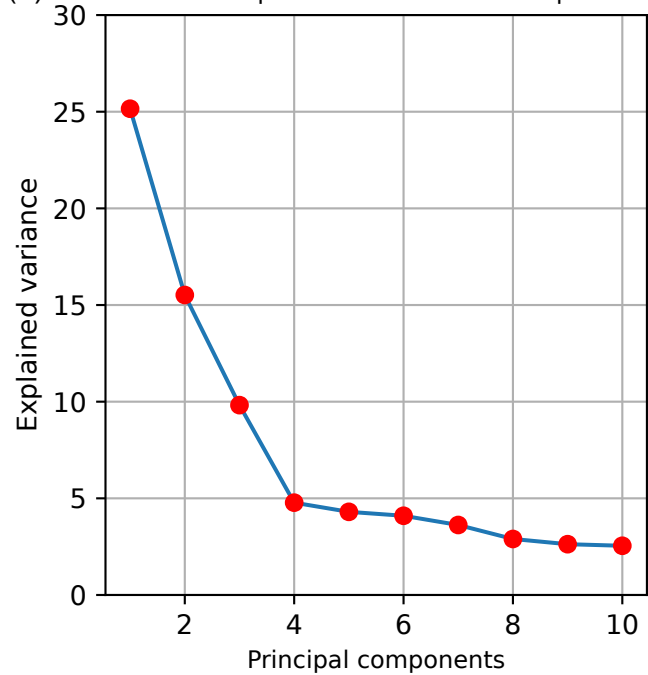
(a) Total 75% explained with first 10 components
