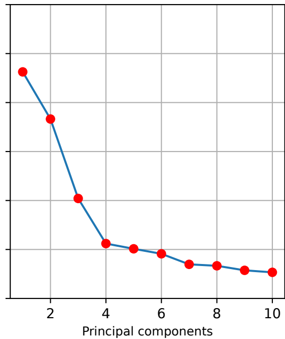
(b) Total 79% explained with first 10 components
