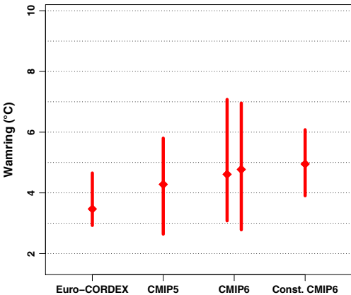
Annual
