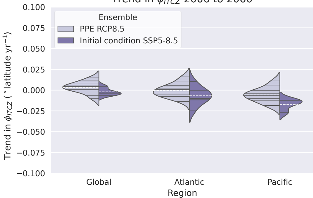
Trend in \phi_{ITCZ} 2006 to 2060
