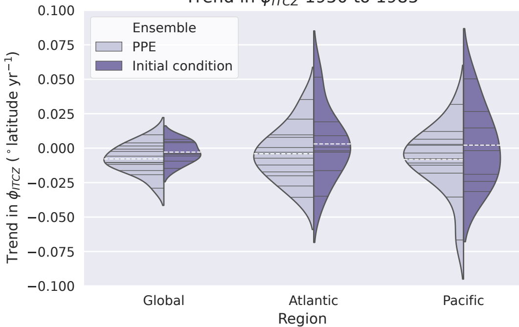
Trend in \phi_{ITCZ} 2006 to 2060
