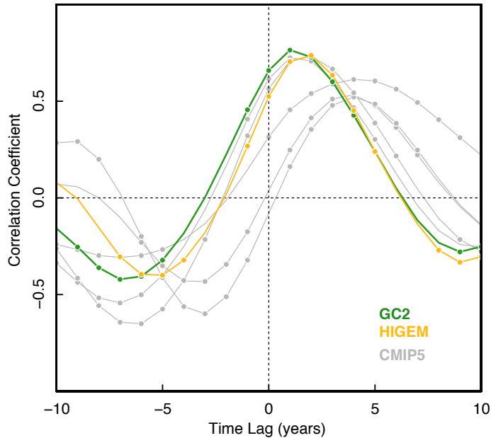
(a) Cross-correlation PC1-LSD vs. OHT45N
