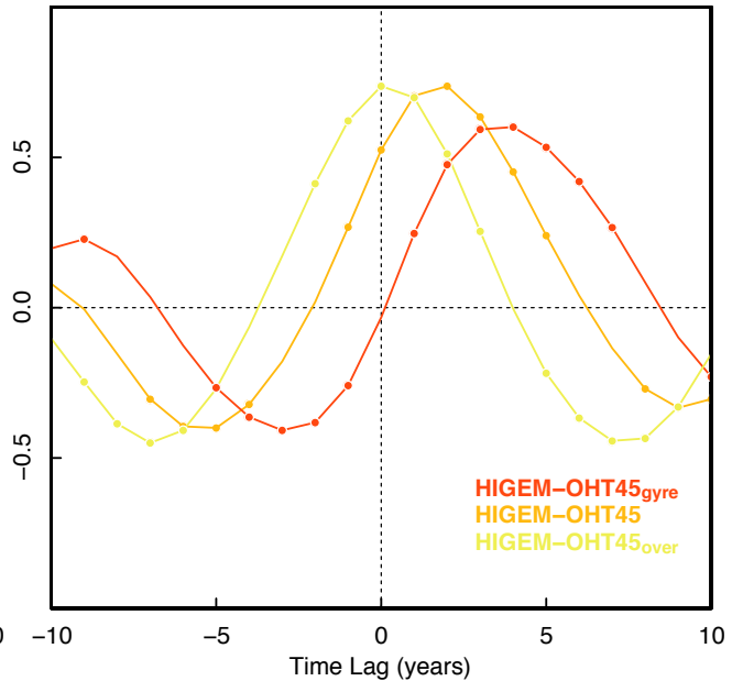
(b) Cross-correlation PC1-LSD vs. OHT45 components
