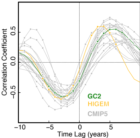
(a) PC1-LSD vs. ESPNA-T700
