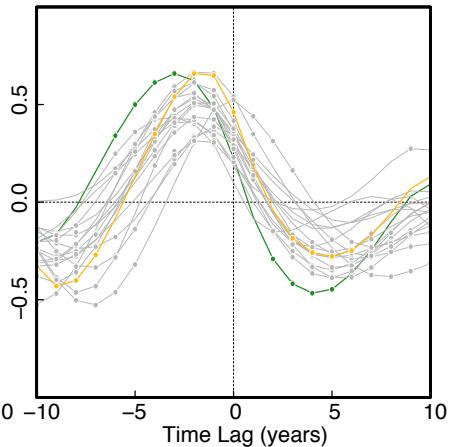
(c) PC1-LSD vs. NAO
