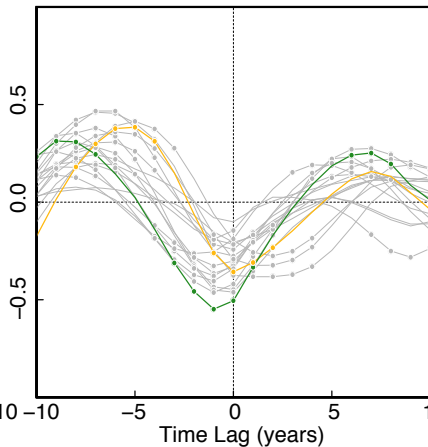
(b) ESPNA-T700 vs. NAO
