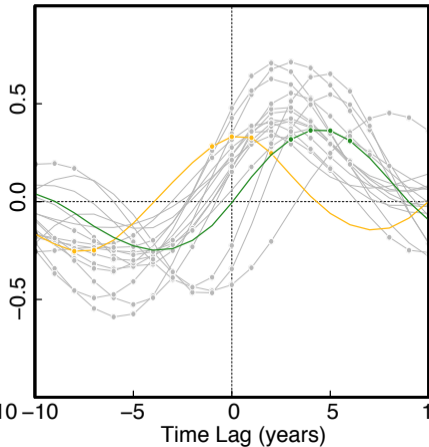
(b) PC1-LSD vs AMOC26
