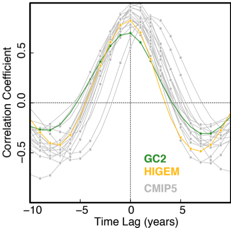
(a) PC1-LSD vs AMOC45
