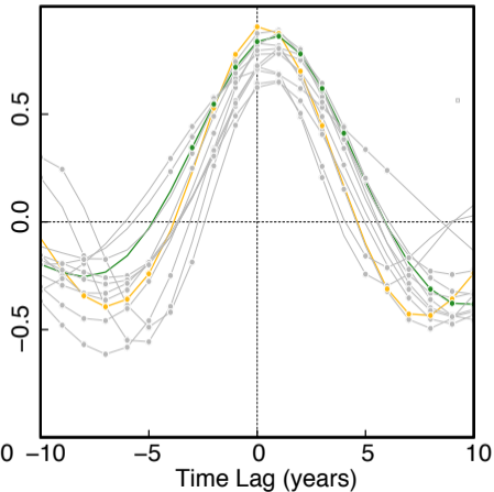
(c) PC1-LSD vs. SPGSI
