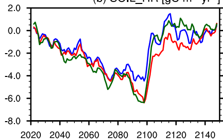
(b) SOIL_HR [ \text{gC m}^{-1} \text{yr}^{-1} ]
