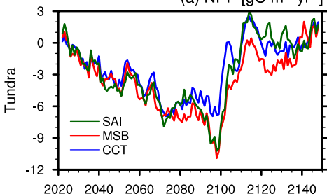
(a) NPP [ \text{gC m}^{-1} \text{yr}^{-1} ]
