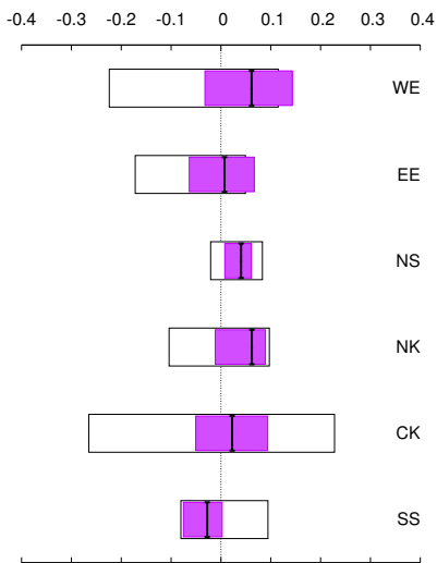
(b) Precipitation
