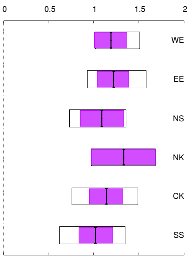
(c) Temperature
