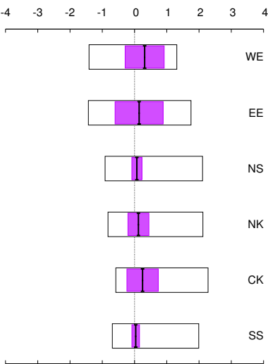
(a) Soil moisture
