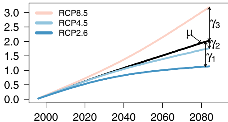
(d) Illustration of the ANOVA for RCP main effects
