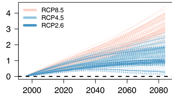
(c) Climate change responses \phi_{i,j,k}^*(t)
