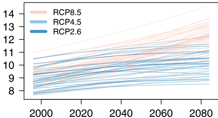
(b) Climate responses \phi_{i,j,k}(t)
