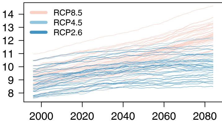
(a) Climate projections Y_{i,j,k}(t)
