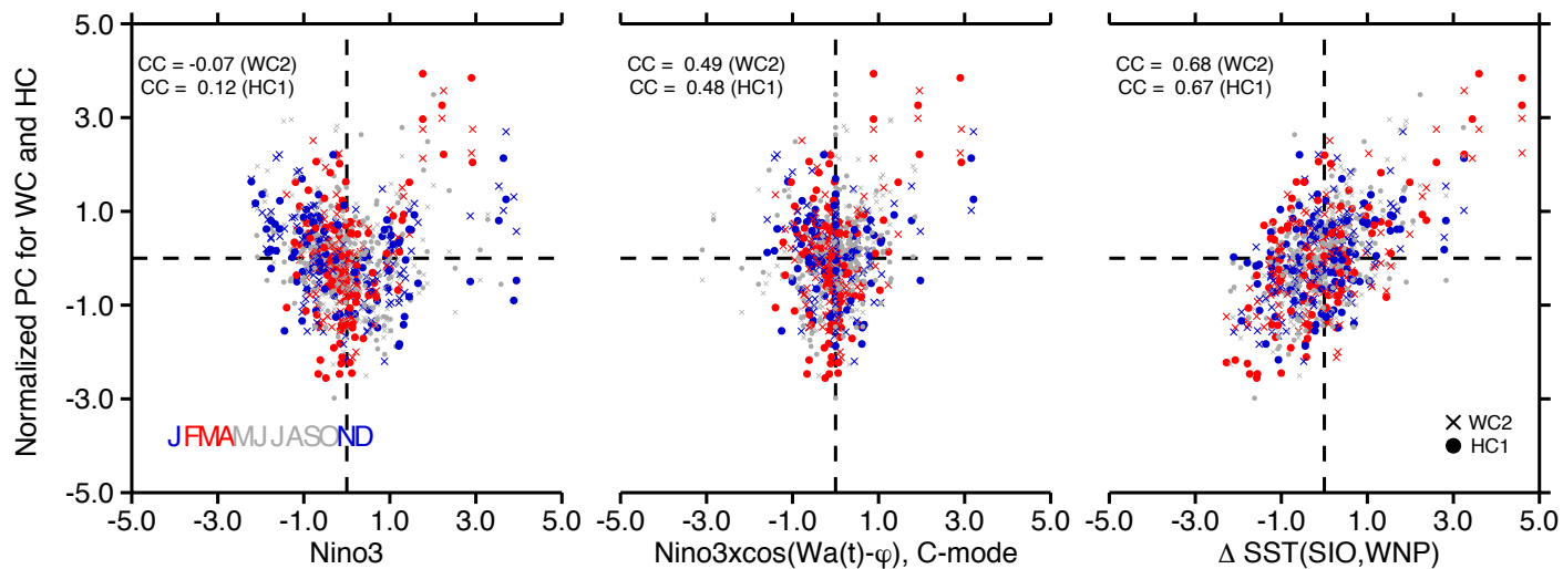
(e) Nino3 vs WC2&HC1 [MME]
