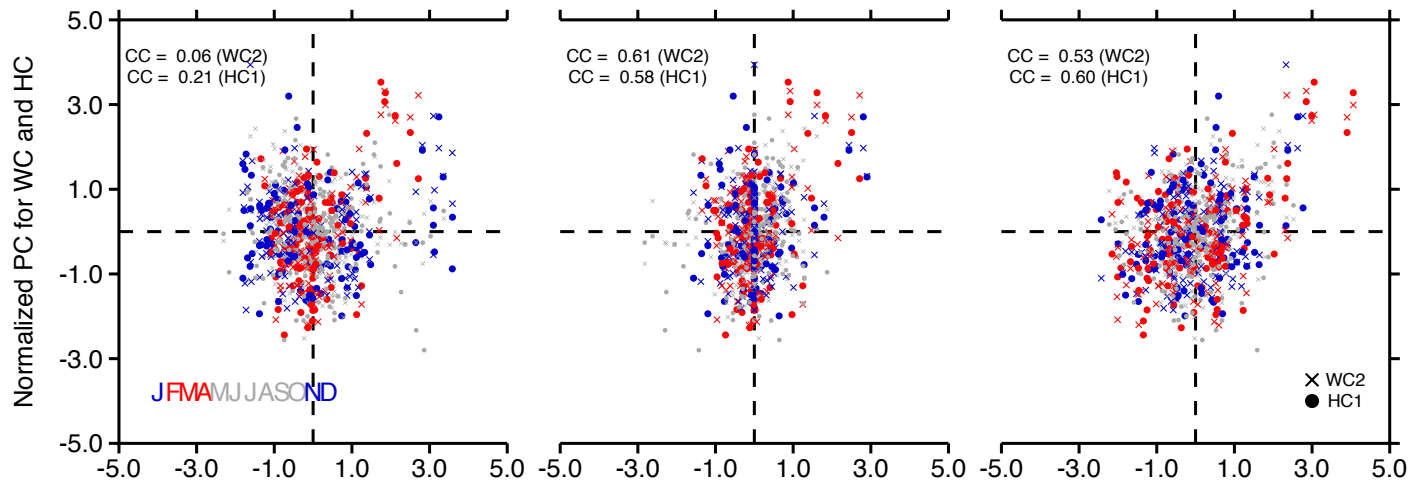
(e) Nino3 vs WC2&HC1 [MME]
