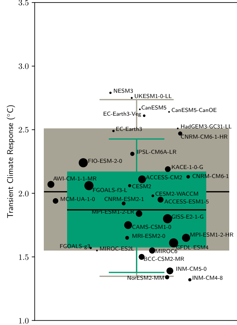
(b) CMIP6 Transient Climate Response
