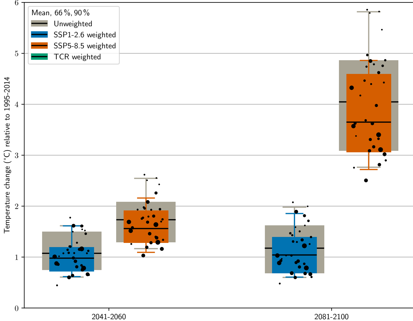
(a) CMIP6 global temperature change
