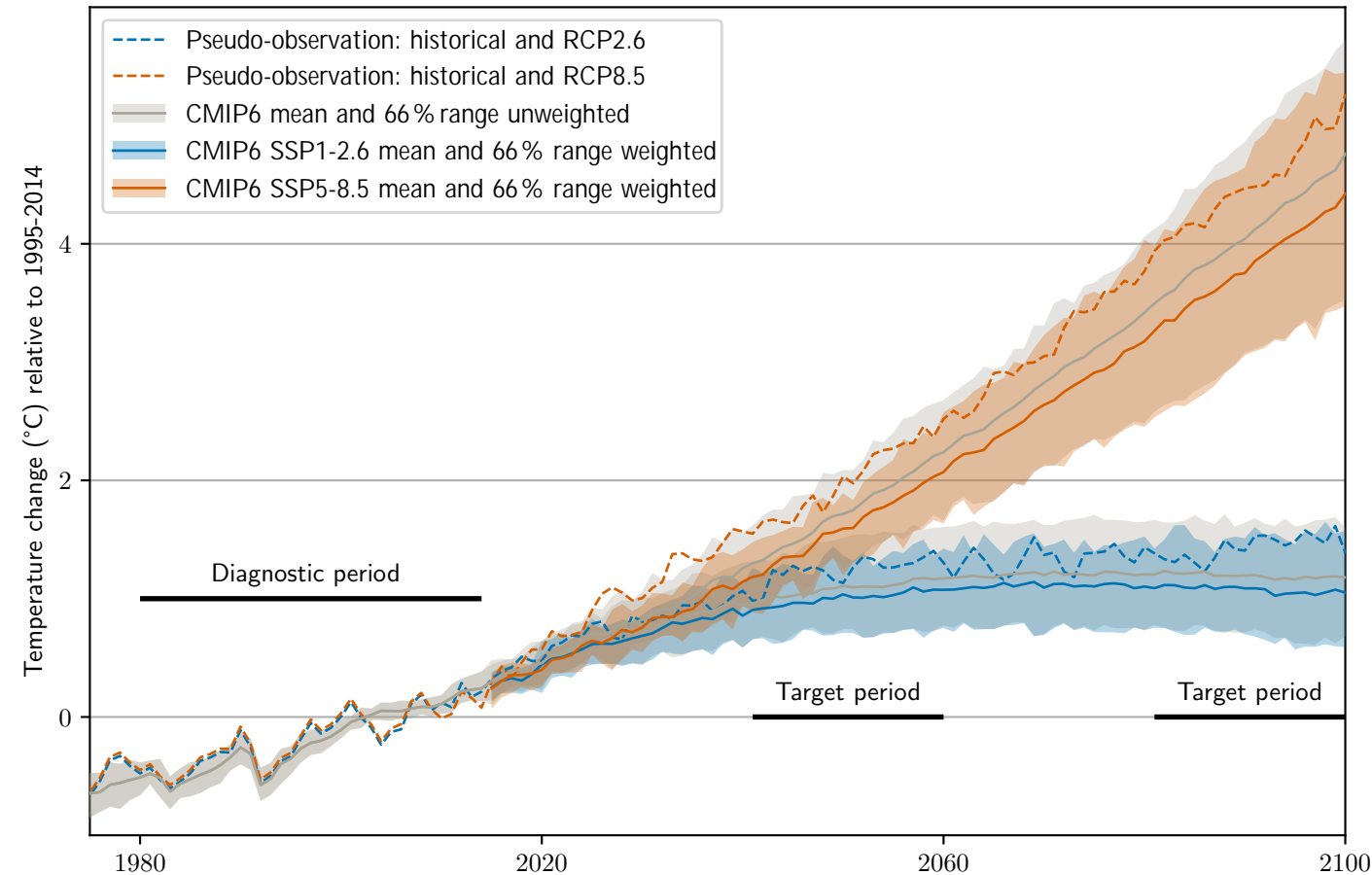
(a) Combined weighting based on pseudo-observations from MIROC-ESM (CMIP5)
