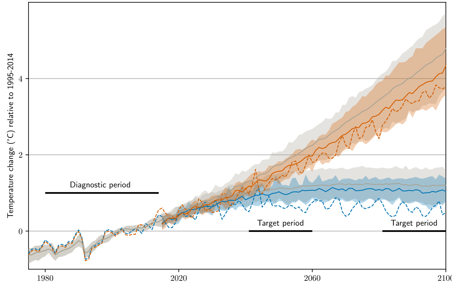
(b) Combined weighting based on pseudo-observations from MPI-ESM-LR (CMIP5)
